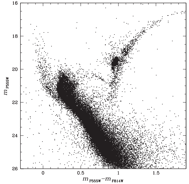
Figure 2. Optical m_{F555W} versus (m_{F555W} - m_{F814W}) CMD for all of the sources detected in the HST field surrounding the stellar cluster NGC 419.
