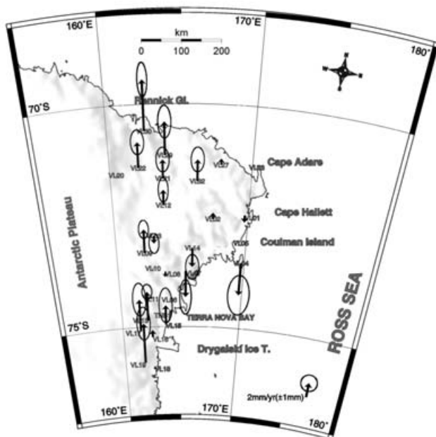
Fig. 6. Vertical motions occurred from December 1999 to January 2003 expressed in \text{mm yr}^{-1} . To avoid plotting misunderstanding for the reader, error ellipses at 95% level of significance are omitted for velocities minor than 1\text{ mm yr}^{-1} .
