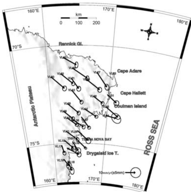
Fig. 4. Planimetrical absolute motions as observed by the analysis of data collected from December 1999 to January 2003. Values in \text{mm yr}^{-1} and error ellipses at the 95% level of significance.
