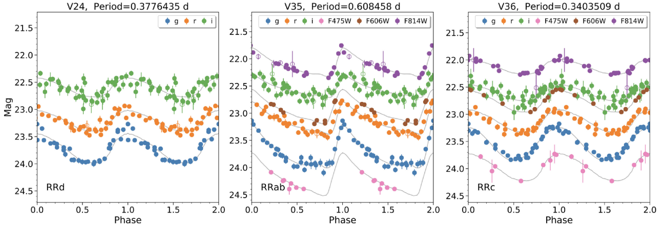
Figure 6. Example of some light curves of the RRL stars discovered in Eri II in the g, r, i (Goodman+DECam) and F475W, F606W, F814W (ACS) bands (when available). The name of the variable and its period are displayed at the top of each panel. Open symbols show the data for which the uncertainties are larger than 3\sigma above the mean error of a given star and, therefore, they were not considered in the period, amplitude and mean magnitude calculations. For clarity, g, i, F475W, F606W , and F814W light curves have been shifted by +0.4, -0.6, +0.7, -0.2 , and -0.6 mag, respectively. Template fits for each light curve are shown by grey lines. All light curves are available as Supporting Information with the online version of the paper. The individual g, r, i, F475W, F606W , and F814W photometry for the variables detected in this work are in Table S1.
