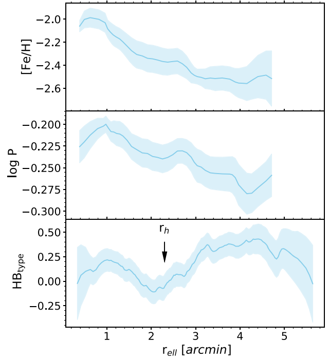
Figure 13. Radial gradient of the metallicity (top), the logarithm of the period (middle), fundamentalized for the RRL types, of the RRL stars in Eri II, and the morphology of the HB ( \text{HB}_{\text{type}} , bottom). The blue shaded areas show the corresponding uncertainties.
