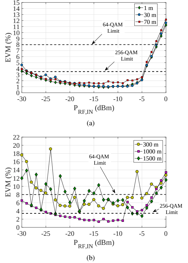
Fig. 5: EVM Measurements of short-range (up to 70 m) (a) and medium-range (up to 1500 m) (b) A-RoF systems.
