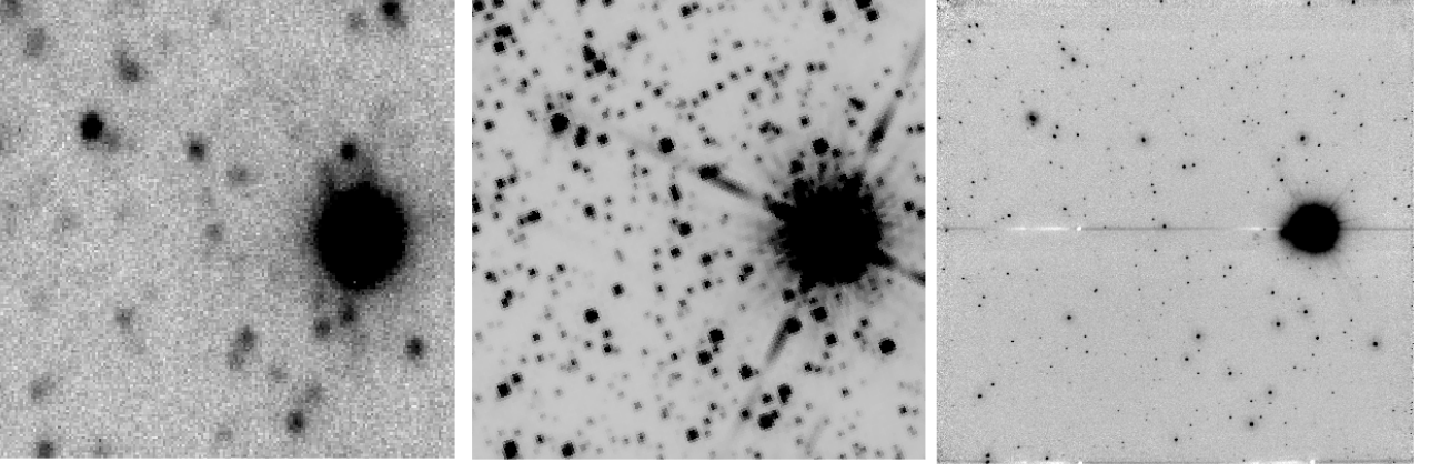
FIG. 2.— The sky region covered by the PISCES camera (right panel) as seen also by LUCI1 (left) and the WFC3 (center). Note the change in spatial resolution, from 0.118''/\text{px} (seeing limited), 0.13''/\text{px} (from space), 0.026''/\text{px} .
