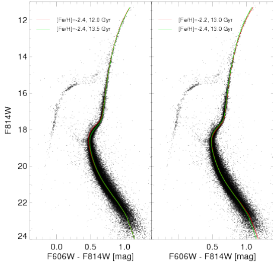
FIG. 7.— Comparison with isochrones of different ages (left) and metallicities (right).
