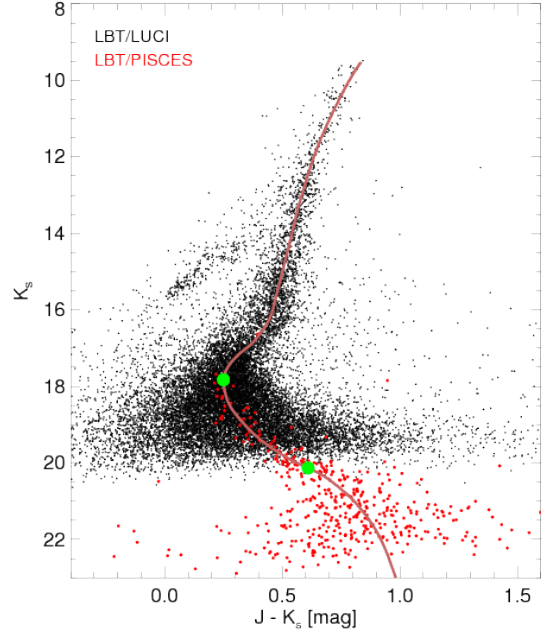
FIG. 8.— (K, J - K) CMDs from LBT data (black: LUCI1; red: PISCES) with superimposed the derived ridge line. The big dots mark the MSTO and MSK points.
