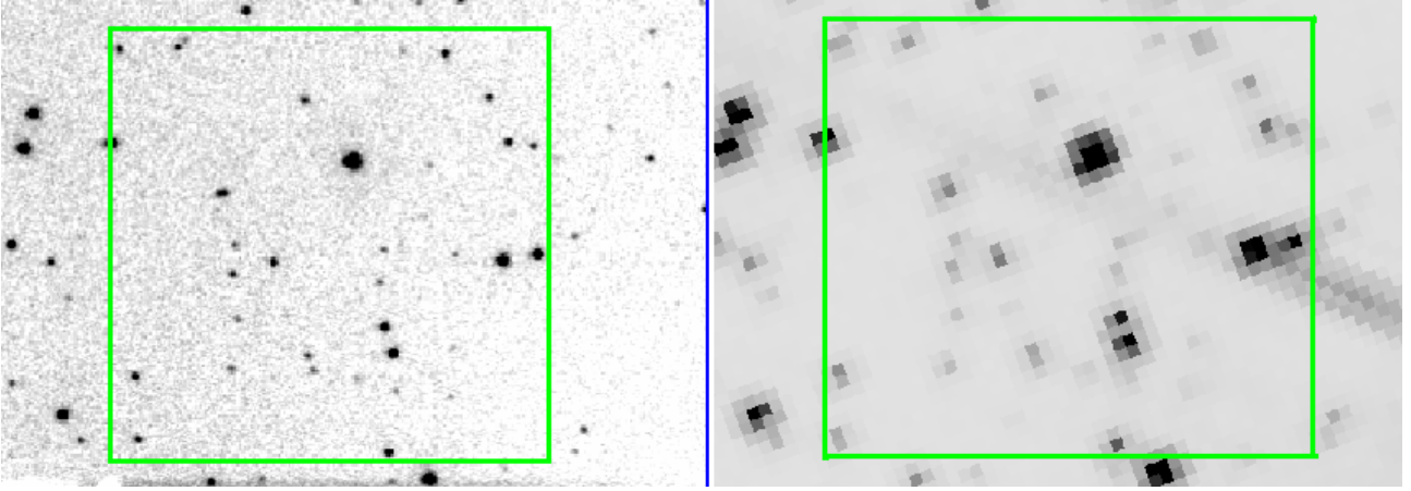
FIG. 3.— A zoom on the same PISCES (left) and WFC3 (right) images of Figure 2. The green square highlights the same sky region of 5'' \times 5'' . The comparison clearly shows the gain in spatial resolution of the PISCES data.
