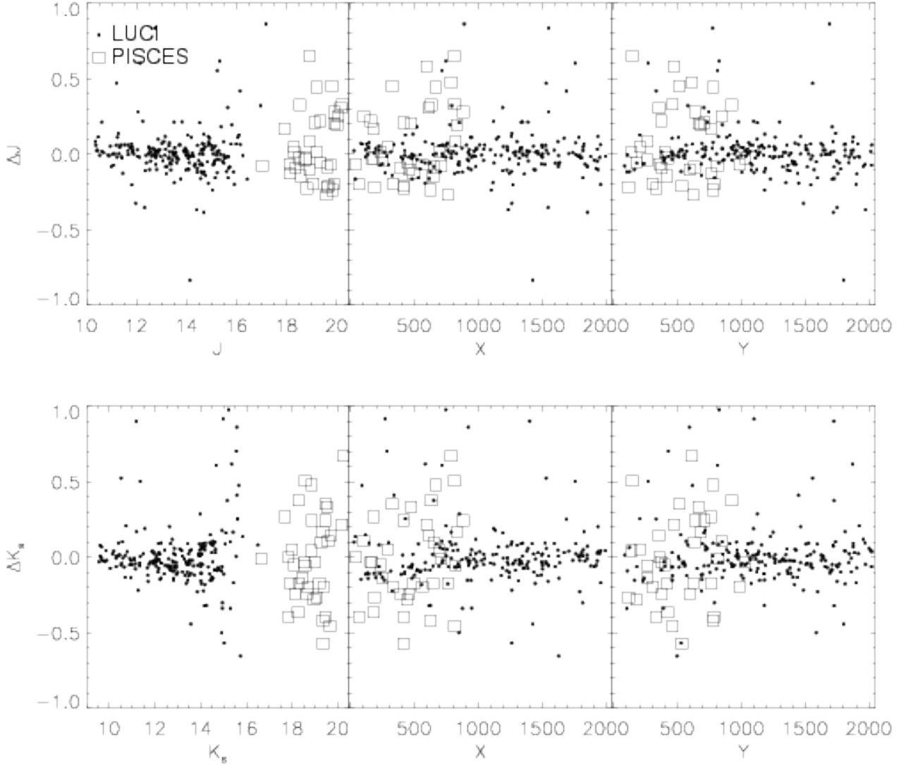
FIG. 4.— Residuals of the calibrations as a function of magnitude ( Left ), X coordinate Center , and Y coordinate Right . top and bottom rows refer to the J and K_s bands, respectively. Large dots show the more than 200 stars in common between the LUCI catalogue and 2MASS. Big open squares compare the \sim 35 stars in common between LUCI1 and PISCES, at significantly fainter magnitude. Note that the range of X and Y are different because of the size of the two cameras.
