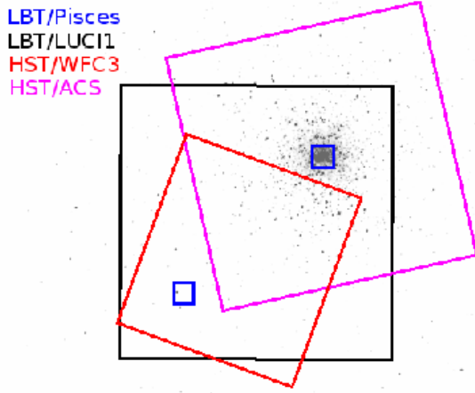
FIG. 1.— SDSS image of M 15 with superimposed the fields of the different data sets collected for this project. Detailed analysis of the central PISCES field will be presented in a forthcoming paper.
