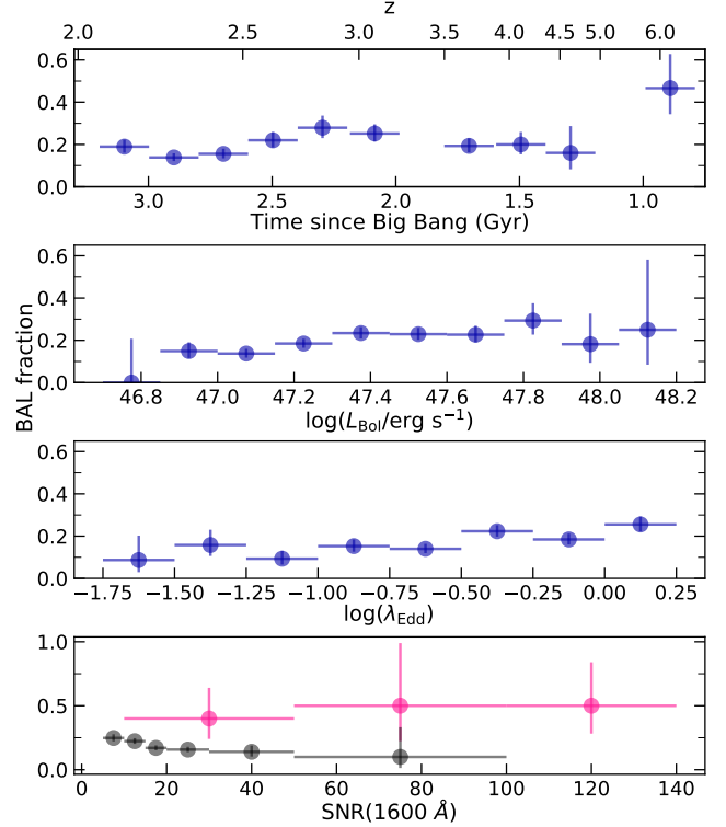
Figure 7. BAL fraction as a function of different physical quantities. Top: cosmic time, from 0.8 to 3.2 Gyr from the Big Bang, in bins of \sim 200 \text{ Myr} . Top axis indicate the corresponding redshift interval. Second from top: quasar bolometric luminosity, estimated from the rest-frame optical via bolometric correction. Second from bottom: accretion rate. Bottom: median SNR of the quasar continuum at rest-frame 1600 \text{ \AA} (Sect. 4). Black(magenta) dots refer the 2.1 < z < 5.0 ( 5.8 < z < 6.6 ) sample. In each panel, horizontal bars indicate the bins in which BAL fractions have been calculated, while vertical bars show Poissonian uncertainties at a 90% confidence level for each bin (Gehrels 1986)
