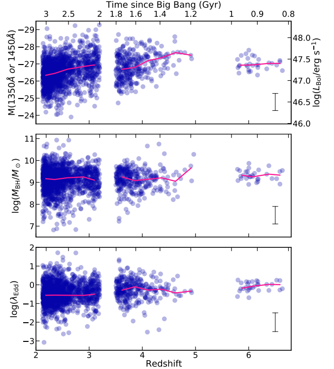
Figure 1. Absolute magnitude (top), BH mass (middle) and Eddington accretion rate (bottom) as a function of redshift for the quasar sample considered in this work. Top axis indicates time since Big Bang. Magenta line represents the median magnitude in redshift bins \Delta z = 0.25 . Error bars represent the typical uncertainties (see Sect. 2.2 and Sect. 2.3)
