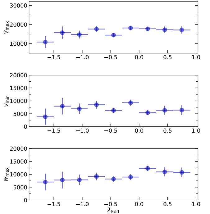
Figure 10. Maximum velocity (top), minimum velocity (middle) and maximum width (bottom) in units of \text{km s}^{-1} , as a function of \lambda_{\text{Edd}} for the C IV BAL outflows in our quasar sample. Horizontal bars indicate the accretion rate bins in which the average BAL velocity has been calculated. Vertical bars indicate the standard deviation error on the average value for each bin
