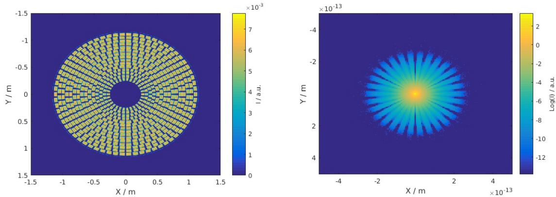
Figure 3. Transverse intensity distributions. Left: Shortly after the optic. The optics structure is clearly reflected in the pattern, including the gap in the middle of the SPO mirror modules. Right: At the focal point (12m). For clarity we plot the \log(I) . The radial structure of the optics is reflected in the pattern, but note that the axis limits \ll \lambda .
