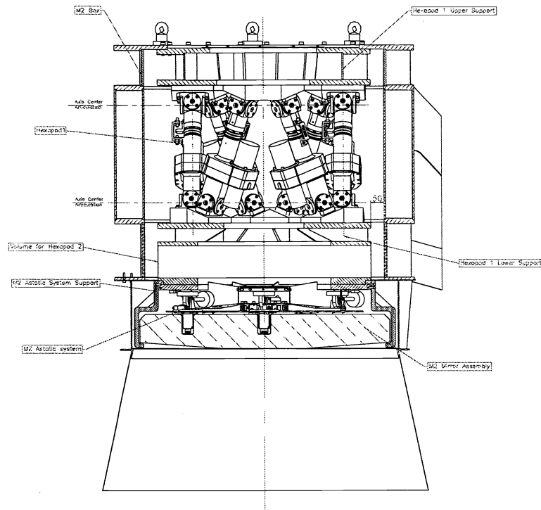
Fig. 4 – A M2 box section view
