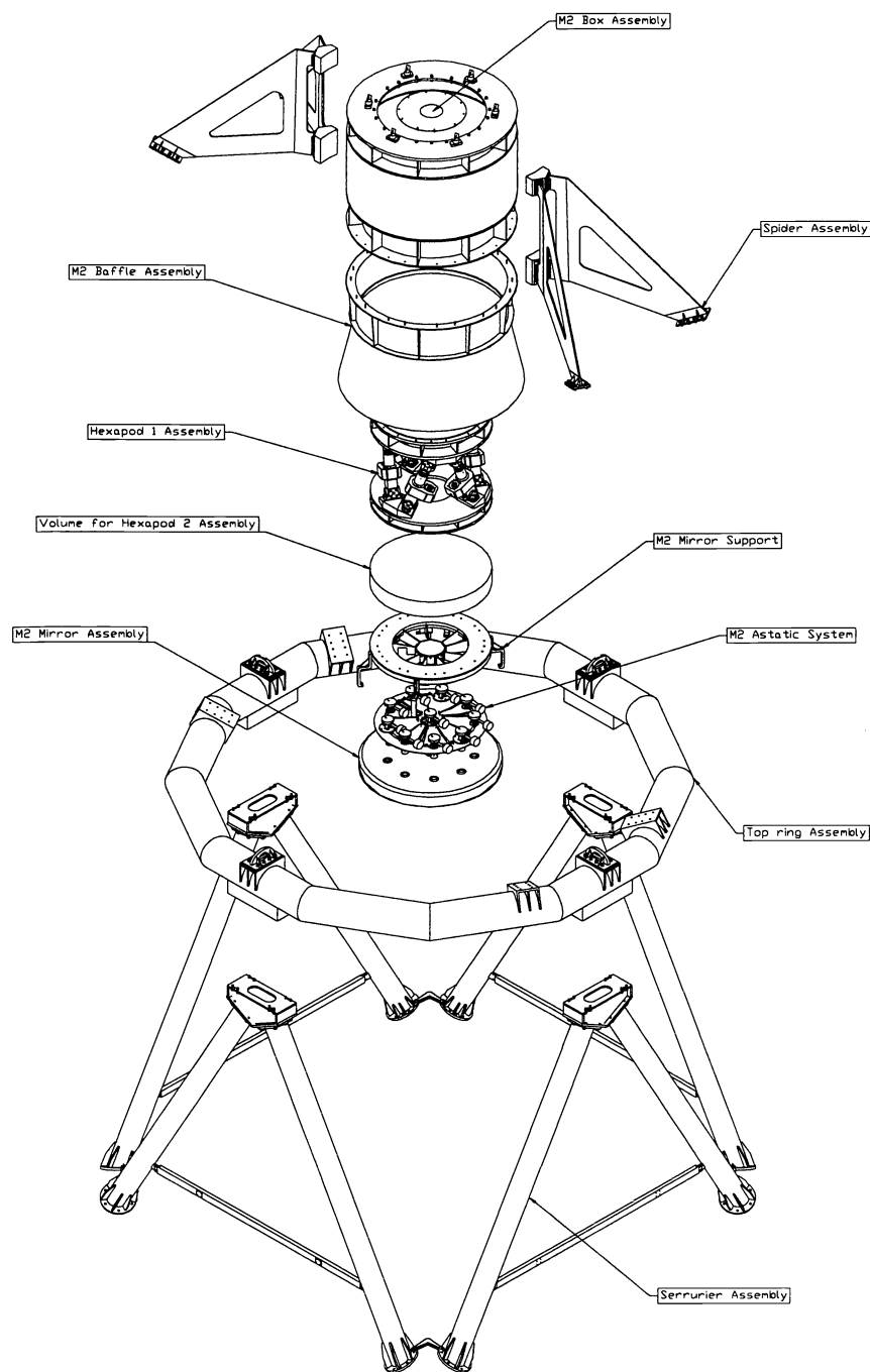
Fig. 3- VST Serrurier and Top Assembly Exploded view
