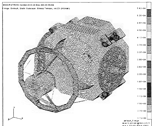
Fig. 12 – Element stress for gravity load applied along y axis, telescope at 90°.
