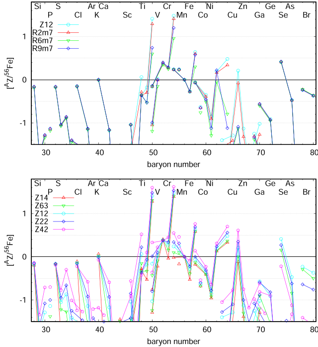
Figure 2. Final composition after radioactive decays for the models with different \dot{M}_{\text{acc}} (top) and Z_{\text{ini}} (bottom): [^A Z / ^{56}\text{Fe}] = \log_{10} [m(^A Z) / m(^{56}\text{Fe})] - \log_{10} [m(^A Z) / m(^{56}\text{Fe})]_{\odot} .
