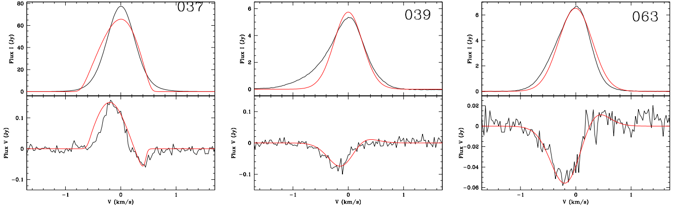
Fig. A.2. Total intensity ( I , upper panel ) and circular polarization intensity ( V , lower panel ) spectra for the \text{H}_2\text{O} maser features 037, 039, 063. The thick red line shows the best-fit models of I and V emission obtained using the FRTM code (see Appendix A). The maser features are centered on zero velocity.
