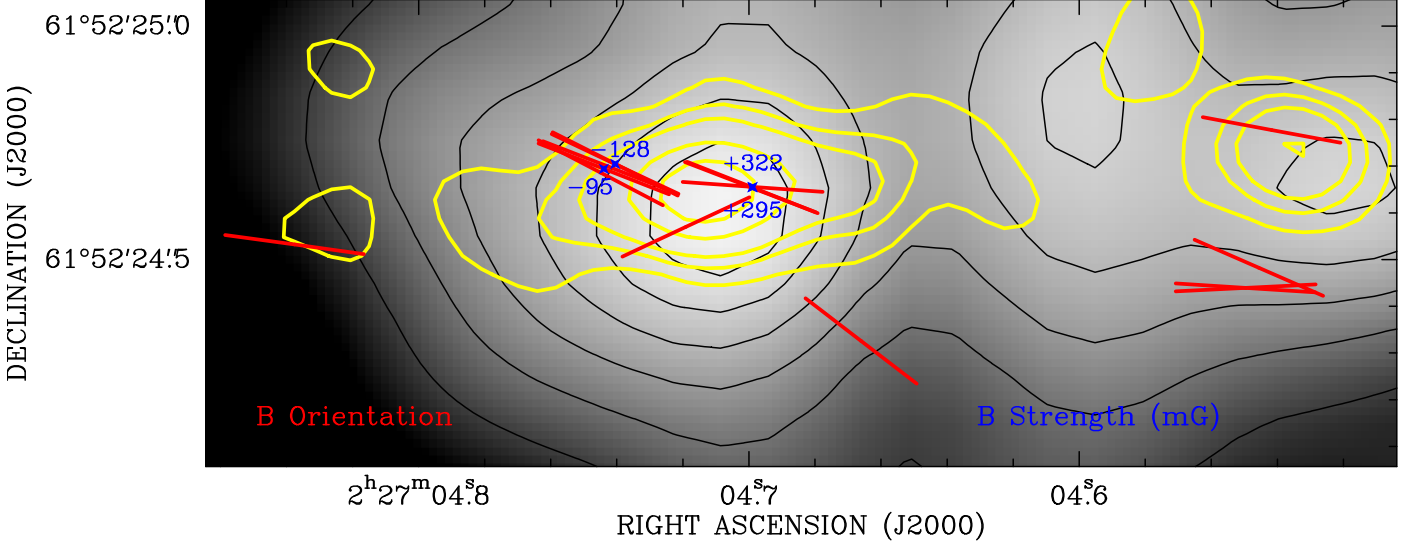
Fig. 2. Magnetic field orientation (in the plane of the sky) for 17 individual masers with P_l < 5\% (red segment) and strength for 4 (non-saturated) masers for which the Zeeman splitting was measured. The 8.4 GHz emission imaged with the VLA (beamsize \sim 0''.2 ) by Wilner et al. (1999) (yellow contours: corresponding to 0.02, 0.06, 0.1, 0.2, 0.3 mJy beam ^{-1} ) is overplotted onto the 1.4 mm continuum emission mapped with the PdBI (beamsize \sim 0''.5 ) by Wyrowski et al. (1999) (gray scale and black contours: same as in Fig. 1). The radio continuum shows a main central component, the synchrotron jet, and two (western and eastern) secondary components (see § 4.1 for an interpretation).
