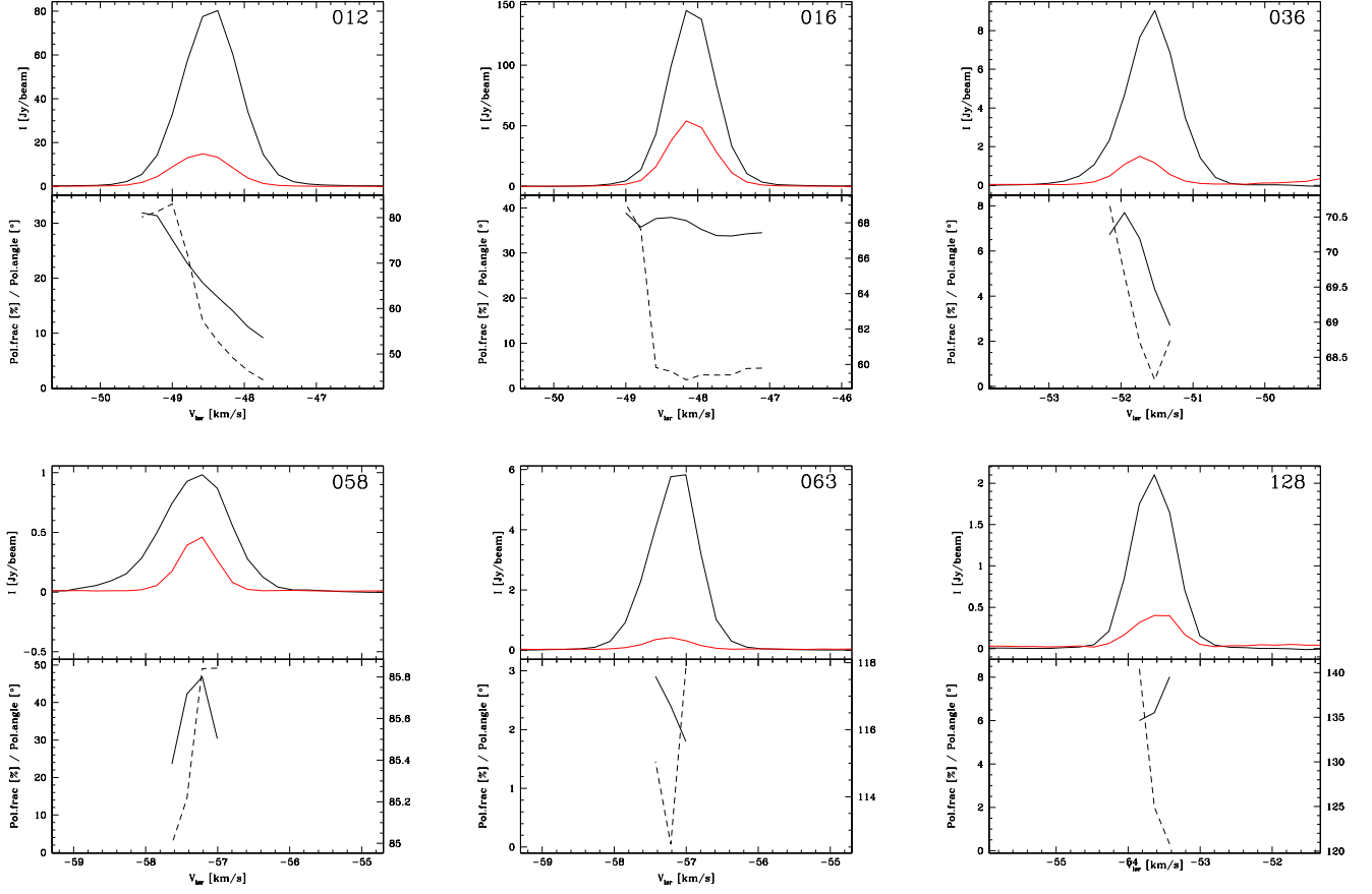
Fig. A.1. Total intensity ( I , black solid line) and linear polarization intensity (red solid line) spectra of the \text{H}_2\text{O} maser features 012, 016, 036, 058, 063, and 128 ( upper panel ). The linear polarization intensity spectra have been multiplied by a factor of three for 036, 063, and 128. The linear polarization fraction (black solid line, left scale) and the linear polarization angle (dashed black line, right scale) are also shown ( lower panel ).
