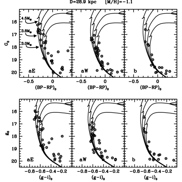
Figure 9. CMDs of the aE, aW and b subsystems (left-hand, central, and right-hand panels, respectively) from Gaia DR2 (upper row of panels) and PanSTARRS1 (lower row of panels) photometry. On each CMD, we overplotted four isochrones at metallicity [M/H] = -1.1 , shifted to the distance of PW 1, with age \simeq 100, 160, 250 , and 400 Myr, from left to right, from the PARSEC set. In the upper left-hand corner we indicated the initial stellar masses corresponding to G_0 = 16.0, 17.1 , and 18.0 on the age = 100 Myr isochrone.
