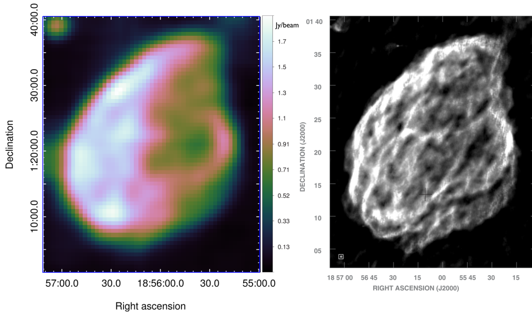
Figure 8. Comparison of the continuum maps of SNR W44 obtained with SRT at 7.0 GHz (left) with that obtained with the VLA at 324 MHz (right) ( Credit: Castelletti et al. 2007, reproduced with permission © ESO ). The beam size in the SRT map is represented by the point-like source in the top left corner.
