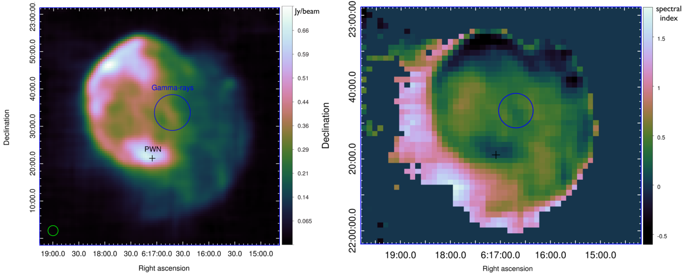
Figure 3. Continuum map of SNR IC443 at 7 GHz (left) and spectral index map obtained by using 1.55 and 7 GHz data (right). The black plus symbol indicates the position of the PWN, whereas the blue circle indicates the bulk of the gamma-ray emission seen with VERITAS (Humensky & the VERITAS Collaboration 2015).
