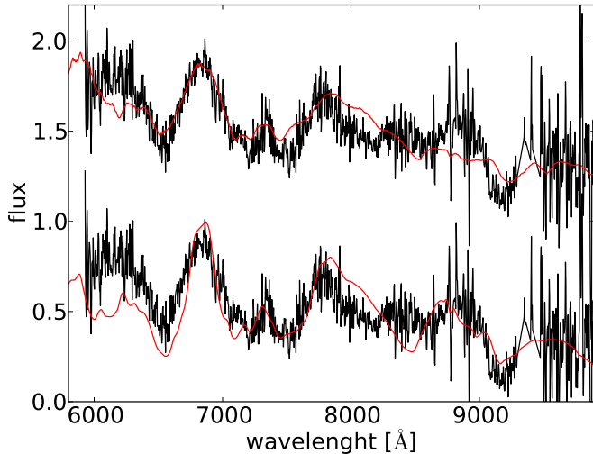
Fig. 4. Observed spectrum of SN 2012gs obtained with FORS2 on MJD 56 252.0 (black line) is compared to that of the SN Ic 2007gr at phase -9d (top) and of the type Ia SN 1991T at phase +14d (bottom). In both cases it is adopted for SN 2012gs at redshift z = 0.5 , as measured from the narrow emission lines of the host galaxy.
