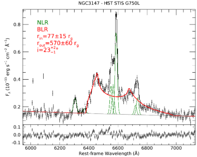
Figure 1 A remarkably prominent and very broad H line profile (in red) is revealed in the HST STIS G750L spectrum of NGC 3147, carrying the signature of a relativistic thin Keplerian disk, with an inner emitting radius of only 77 r g . Narrow lines from the NLR are in green, the continuum in grey. The fit residuals are shown in the bottom panel.
