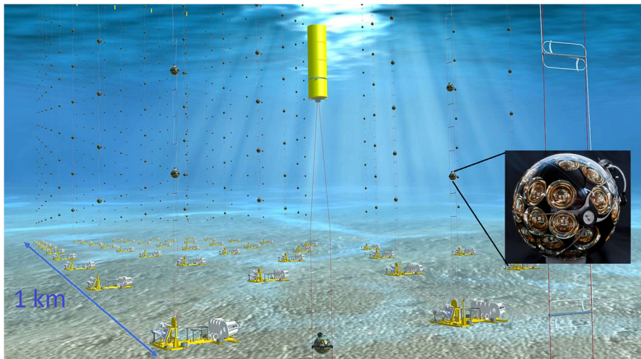
Fig. 9 Schematic view of a neutrino telescope. An array of photo sensors is embedded in a large volume of a transparent medium (water or ice) to determine the direction and energy of secondary charged particles induced by neutrino interactions using the Cherenkov radiation. The figure shows the layout of the KM3NeT detector, in construction in the Mediterranean Sea with one of the multi-PMT sensor (credit: KM3NeT Collaboration, km3net.org)
