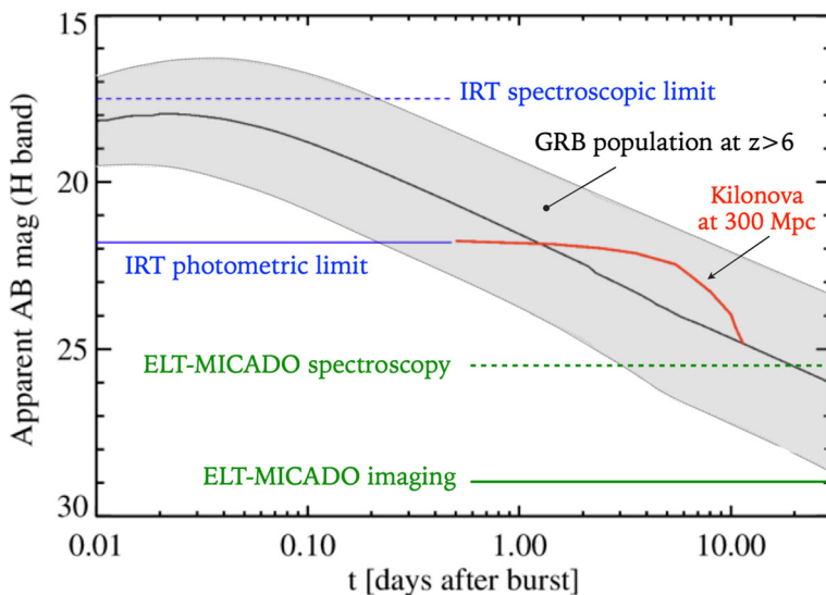
Fig. 3 Expected H-band light curves of the afterglow of high redshift GRBs and a kilonova from NS-NS merger at 300 Mpc. The shaded area indicates the median (black line) and 1\text{-}\sigma scatter of 100 simulated light curves drawn from GRB population models at z > 6 following [11]. The red curve represents the kilonova associated to GW170817, projected to a distance of 300 Mpc, using H-band photometry from [12]. Horizontal lines indicate the limiting magnitude of THESEUS IRT (600s and 1800s exposure for photometric and spectroscopic limit, with SNR= 5 and 3, respectively,) and ESO ELT-MICADO (1 h exposure with SNR = 5) in imaging and spectroscopic mode respectively (re-adapted from [13])
