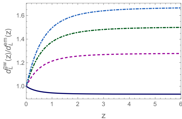
Fig. 8 Example of the ratio of the gravitational to electromagnetic luminosity distance in a modified gravity model, for different values of a parameter related to the energy scale of inflation. In the upper curve, the deviations of d_L^{\text{gw}}(z) from d_L^{\text{em}}(z) reaches 60% at large redshift (from [69])
