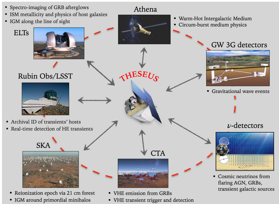
Fig. 1 THESEUS will work in synergy on a number of themes (bullets) with major multi-messenger facilities in the 2030s and will provide targets and triggers for follow-up observations with several of these facilities
