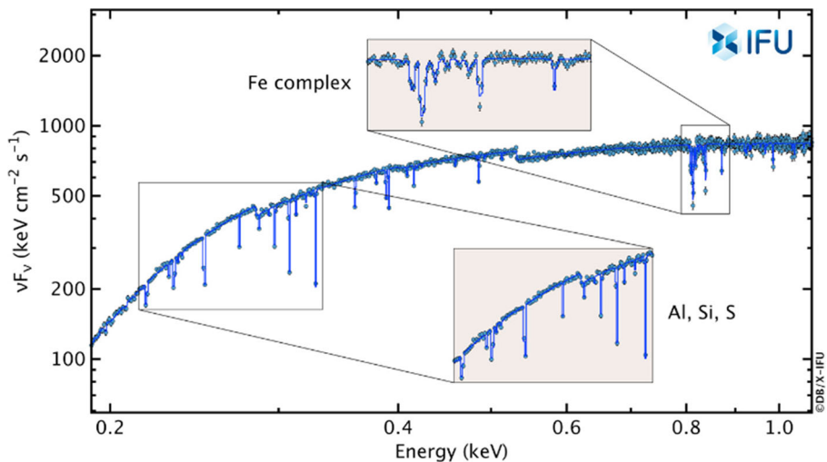
Fig. 2 A simulated Athena/X-IFU spectrum of a medium bright (fluence: 4 \times 10^{-7} erg cm ^{-2} ) z = 7 GRB afterglow characterized by deep resonant lines from the ISM of the GRB host galaxy. An effective intrinsic column density of 2 \times 10^{22} cm ^{-2} was assumed [credit: Athena/X-IFU Consortium]
