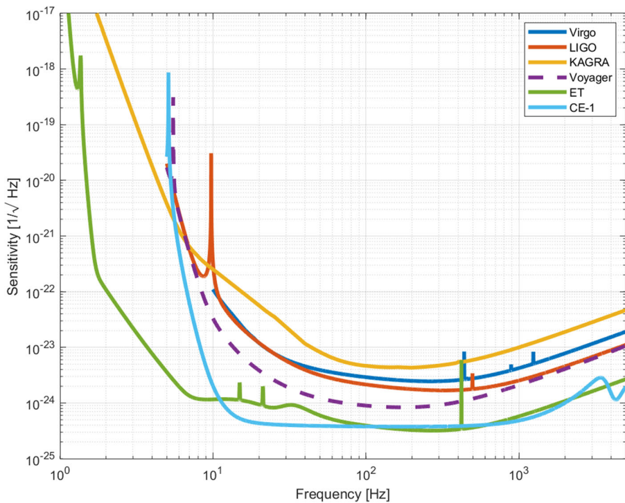
Fig. 5 Strain sensitivities as a function of frequency for the next generation of GW observatories, ET [50] and CE Phase I [45] with respect to the sensitivities of the upgraded instruments of the existing LIGO, Virgo and Kagra expected to be operational in 2025 [47], and LIGO Voyager [48], a possible major upgrade of the LIGO inteferometers in the late 2020s
