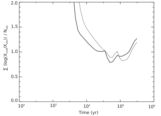
Figure 2. Mean logarithmic difference between the modeled and observed abundances over all observed species (see text) as a function of time using kida.uva.2011 (solid line) and kida.uva.2014 (dashed line).
