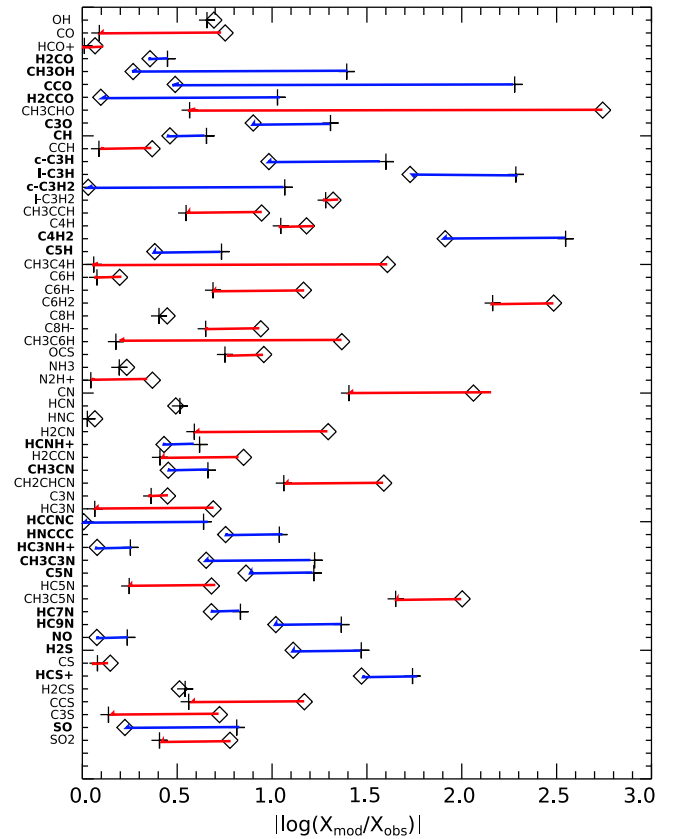
Figure 3. Absolute logarithmic difference between modeled and observed abundances for each species at the best time of each model using plus signs for kida.uva.2011 and diamonds for kida.uva.2014. Horizontal lines show the differences between the old and new values. Red lines indicate that the difference has been increased by the new network while blue lines indicate that it has been reduced. Boldface species are those with abundances improved by the new network.
