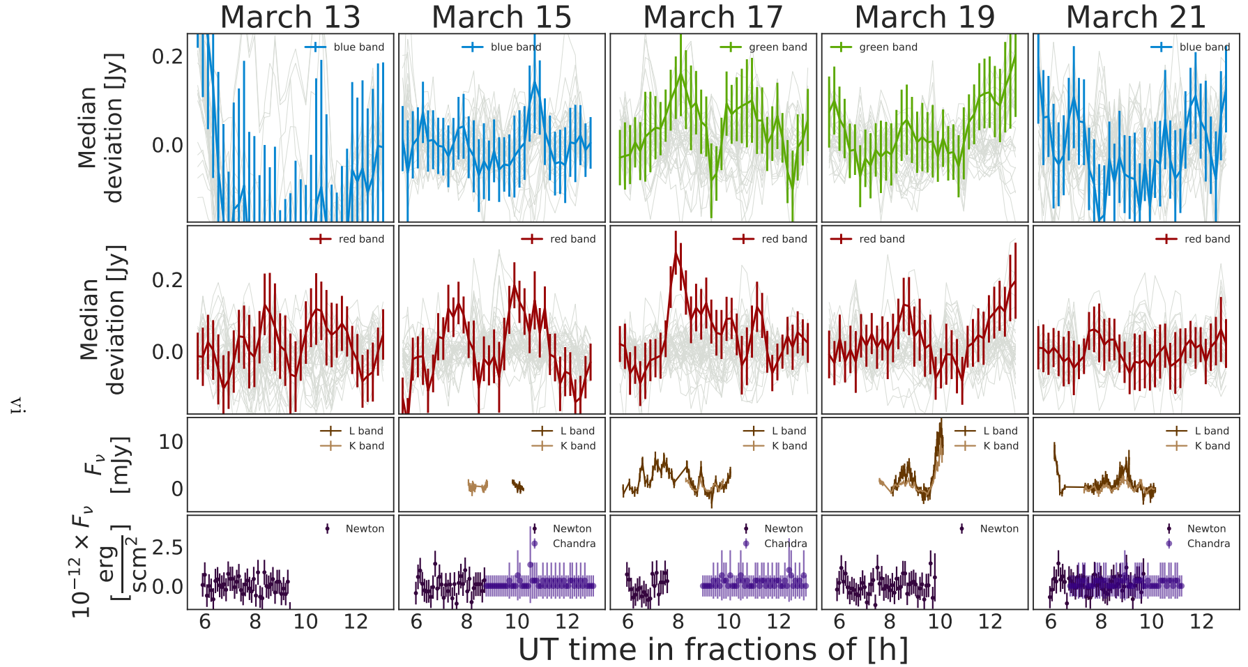
Figure 14: All available light curves. The top two panels show the FIR light curves obtained with Herschel/PACS. The top row are the light curves of the blue and green band (color coded). The panel below is the light curve of the red band. The grey light curves are the light curves of the reference positions (see Section 2.3.1). The lower two panels show the NIR (L' and K band) and X-ray parallel observations from NACO, XMM-Newton and Chandra, where available.
