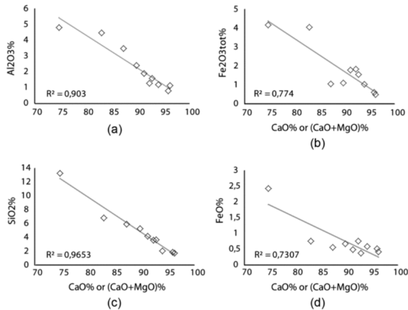
Fig. 8 Variations of (a) Al 2 O 3 , (b) total iron Fe 2 O 3 , (c) SiO 2 and (d) FeO concentrations with (CaO + MgO) amount assumed as representative of the CO 3 2- functional group in carbonate and carbonate–silicate samples. R 2 : coefficient of determination. See also Table 3.
