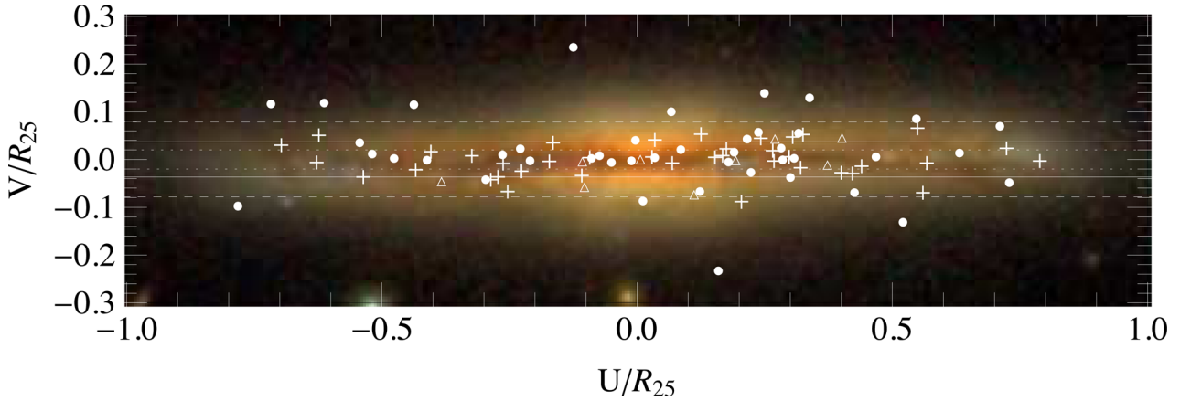
Figure 5. Distribution of coordinates of SNe along the major ( U/R_{25} ) and minor axes ( \tilde{z} \equiv V/R_{25} ) of their Sa–Sd host galaxies. Circles, triangles and crosses, respectively, show Types Ia, Ibc and II SNe. 1\sigma intervals of the distributions of the \tilde{z} coordinates for Type Ia and CC (Ibc+II) SNe are presented by dashed ( \sigma = 0.078 ) and solid ( \sigma = 0.037 ) lines, respectively. The background SDSS image shows the PGC 037591 galaxy (scaled to the distribution), which is one of the representatives of the edge-on galaxies with a prominent dust line along the major axis. Dotted lines show the |\tilde{z}| \leq 0.02 opaque region.
