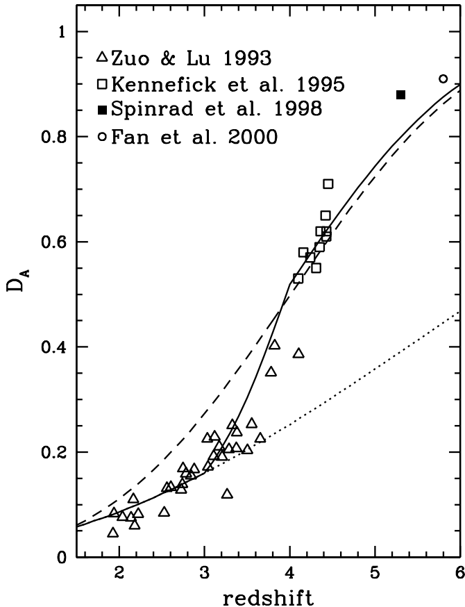
Fig. 2. The deficit D_A in quasar fluxes due to the accumulated absorption of the Ly \alpha forest. The dashed line is obtained by describing the IGM opacity according to the prescriptions by Madau (1995), while the dotted line are those by Scott et al. (2000). The solid line is the model adopted in this paper. References for the data points are indicated. The small difference between the Madau values of D_A and ours at z > 4 is due to the contribution of Ly limit systems (Madau 1995, Eq. (13)), which was not included in Madau's formulation.
