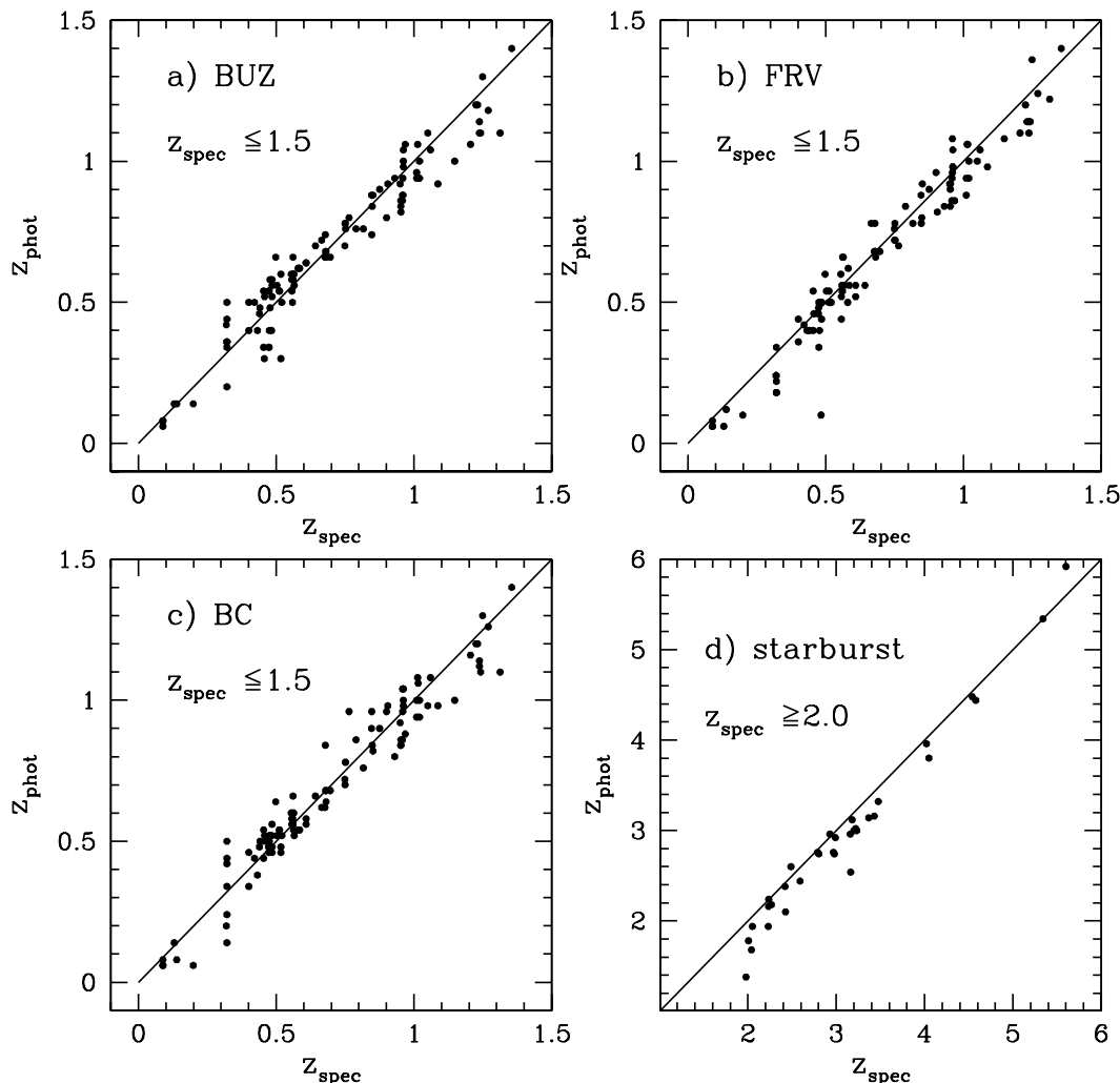
Fig. 1. Comparison between spectroscopic and photometric redshifts according to different template libraries (see the text for acronyms). The solid line is for \Delta z = 0.0 . Note the different scale for panel d).
