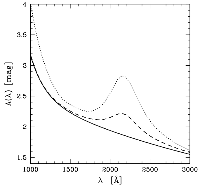
Fig. 5. Differential dust absorption (for E(B - V) = 0.2 ) according to Calzetti's law (solid line), a superposition of Calzetti's law with a 2175 Å bump of amplitude \alpha = 0.25 (dashed line), and the Seaton (1979) extinction curve for the Milky Way (dotted line).
