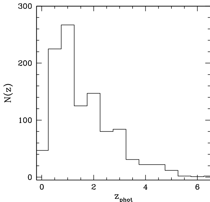
Fig. 9. The redshift distribution of HDFN galaxies.
