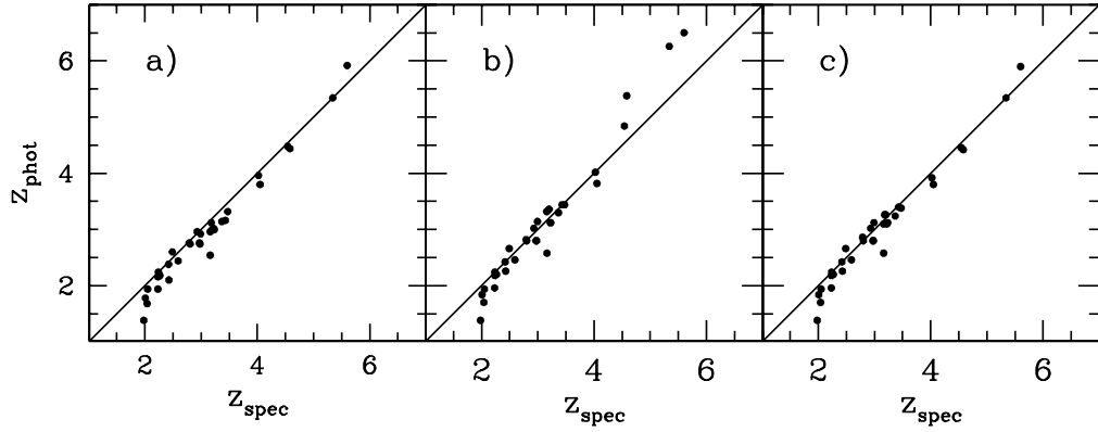
Fig. 3. Comparison between spectroscopic and photometric redshifts at z_{\text{spec}} \geq 2 . Panel a) the IGM opacity follows the prescription by Madau (1995); panel b) by Scott et al. (2000); panel c) the formulation discussed in this paper. The solid line is for \Delta z = 0.0 . It should be noted that when the Scott et al. (2000) results are adopted, the IGM opacity is underestimated at z > 3.5 , and, as a consequence, photometric redshifts overestimate the spectroscopic ones.
