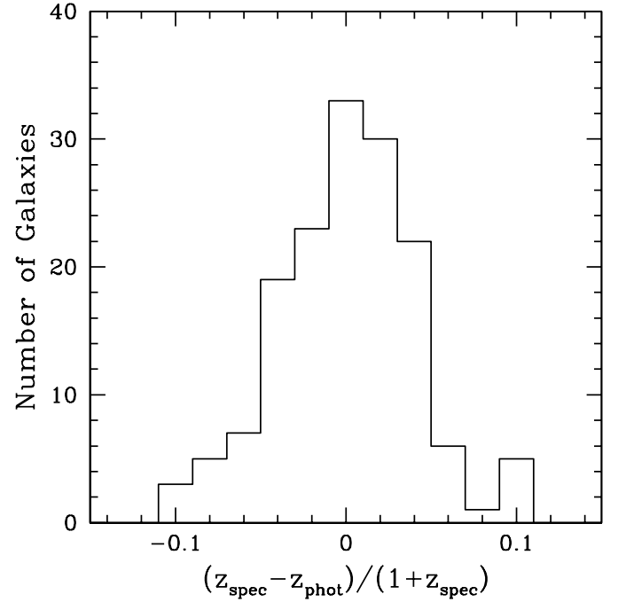
Fig. 8. The distribution of residuals between z_{\text{spec}} and z_{\text{phot}} , normalized to (1 + z_{\text{spec}}) .
