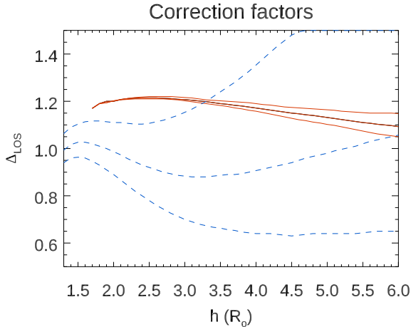
Fig. 4. Radial profiles of correction factors \Delta_{\text{LOS}} as derived for coronal streamers (solid red lines) and coronal holes (dashed blue lines). For each profile the upper and lower curves show the values of the \Delta_{\text{LOS}} parameter resulting from introducing a \pm 5\% error on the measured velocities.
