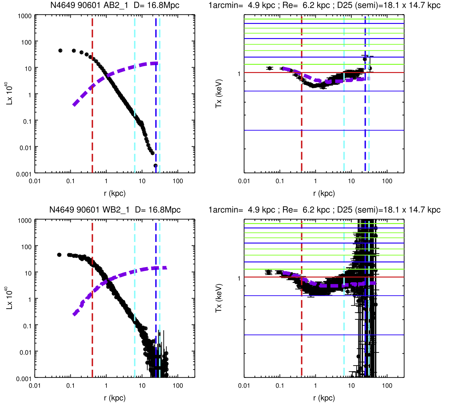
Figure 6. Radial profiles of (left) the surface brightness ( L_{X,GAS} from a given bin in 10^{40} \text{ erg s}^{-1}/\text{area} of the bin in \text{arcmin}^2 ) and (right) the gas temperature in two spatial binning methods, (top) AB and (bottom) WB. The thick dashed purple lines indicate (left) L_{X,GAS}(<r) in 10^{40} \text{ erg s}^{-1} and (right) L_X -weighted mean T(<r) . The vertical lines indicate r = 5 \text{ arcsec} (red), r = 1 and 5 \times R_c (cyan) and r = R_{MAX} (blue), which is the maximum radius where the hot gas is reliably detected with an azimuthal coverage larger than 95% (see Section 5.2).
