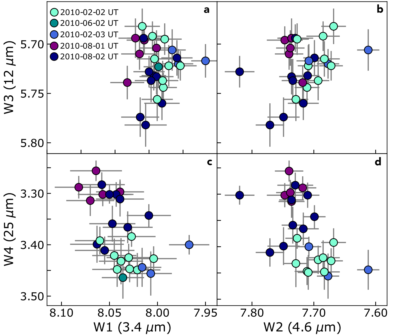
Extended Data Fig. 6 | WISE Time-series photometry of PDS 70. Errorbars represent 1 \sigma . a–b, WISE 3 (W3) is not anticorrelated with WISE 1 and WISE 2 due to the dominant 10 \mu\text{m} silicate emission which does not vary substantially
