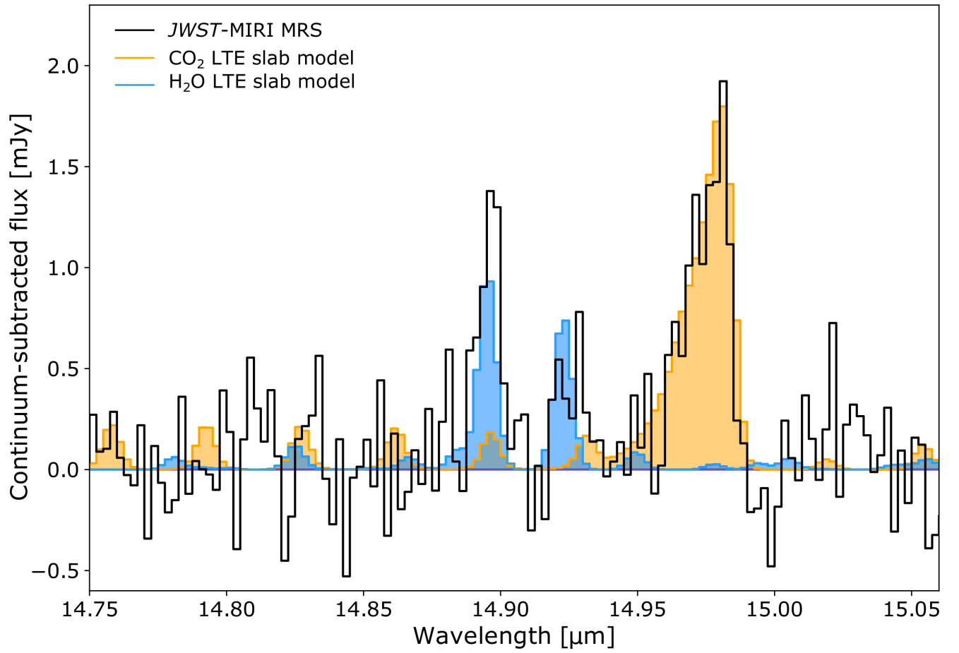
Extended Data Fig. 5 | Continuum-subtracted spectrum in the 15 \mu\text{m} region showing the detected Q-branch of CO 2 (orange). The shape of this feature is sensitive to temperature and is well-fitted by an LTE slab model with T \approx 200 K. The strength of this feature can be reproduced with N(\text{CO}_2) = 1.5 \times 10^{17} \text{ cm}^{-2} and R = 0.1 \text{ AU} . However, the aforementioned parameters are degenerate and are
