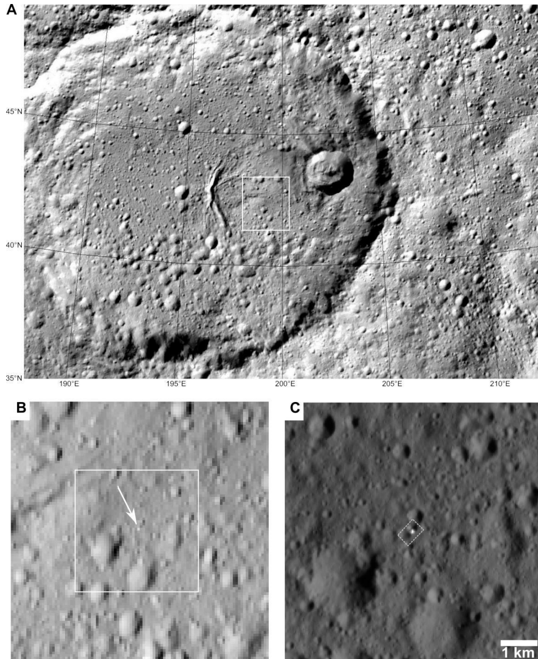
Fig. 11: FC imagery context of the H 2 O-rich material area at 42.20°N, 199.51°E within the Ezinu crater (Combe et al., 2017). A – Mosaic displayed in Lambert conformal conic projection. The white rectangle delimits the close-up view on the right. B – Close-up view from the earliest observation of the high-albedo area (white arrow) with FC from HAMO: unprojected portion of FC21B0042226_15245075026F1E. C – Framing Camera LAMO unprojected portion of FC21B0052773_16021091525F1E of the H 2 O-rich material area at 42.20°N, 199.51°E. The polygon indicates the footprint of the VIR pixels. Data information and scale are provided in Table 3.
