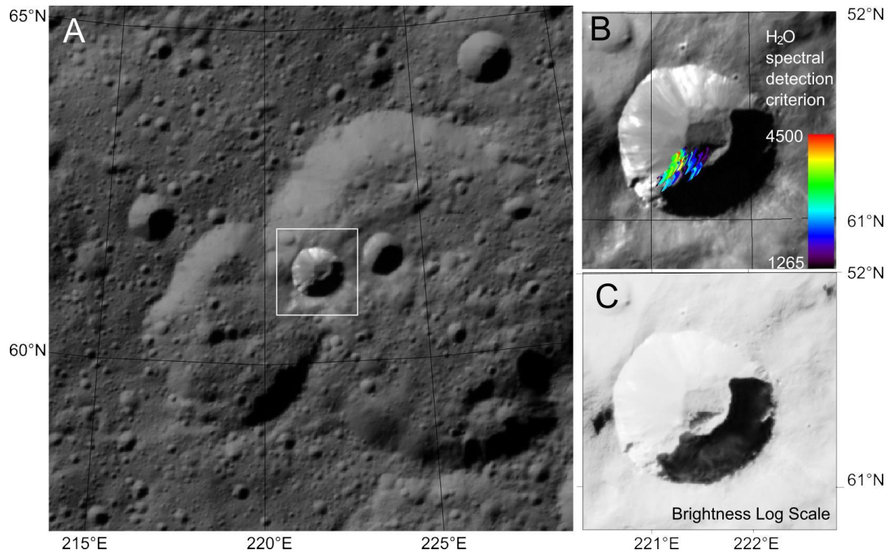
Fig. 8: FC imagery context of the H 2 O-rich material area at 61.32°N, 221.06°E inside a fresh impact crater included in Messor Crater (Combe et al., 2017). A – Mosaic from HAMO observations displayed in Lambert conformal conic projection. The white rectangle delimits the close-up view on the right. B – Close-up view of the fresh crater from image FC21A0047863_15358091114F1G acquired from LAMO. Colored pixels represent VIR H 2 O detections of H 2 O from LAMO. Values are mixing coefficient divided by the RMS (i.e., the quantity that was used to identify H 2 O from VIR spectra). C – Same FC image as B, with brightness display stretched in logarithmic scale in order to visualize both illuminated and shadowed areas.
