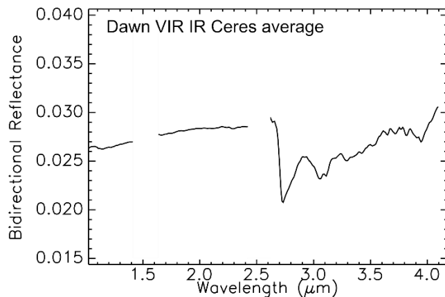
Fig. 1: Ceres average IR spectrum measured by Dawn's VIR IR imaging spectrometer (De Sanctis et al., 2015).
