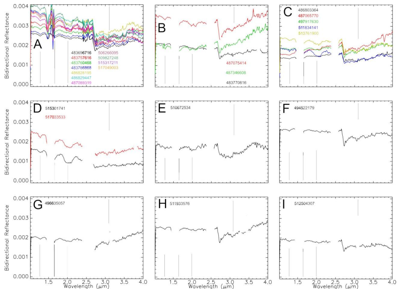
Fig. 4: Average bidirectional reflectance VIR IR spectra of all H 2 O-rich areas identified on Ceres. Vertical gray lines indicate expected locations of H 2 O absorption bands at 1.28, 1.65 and 2.0 \mu\text{m} , as well as the position of the Fresnel peak of crystalline H 2 O ice 3.1 \mu\text{m} . The number of pixels per average spectrum is documented in Table 2. A – (41.42°N, 0.76°E) Oxo Crater. B – (69.66°N, 114.81°E). C – (61.32°N, 221.06°E). D – (-34.83°N, 168.99°E) Juling Crater. E – (61.57°N, 51.82°E) Flow feature (Schmidt et al., 2017). F – (29.60°N, 155.07°E). G – (-47.92°N, 265.46°E) Baltnay Catena. H – (42.20°N, 199.51°E). I – (44.61°N, 32.50°E).
