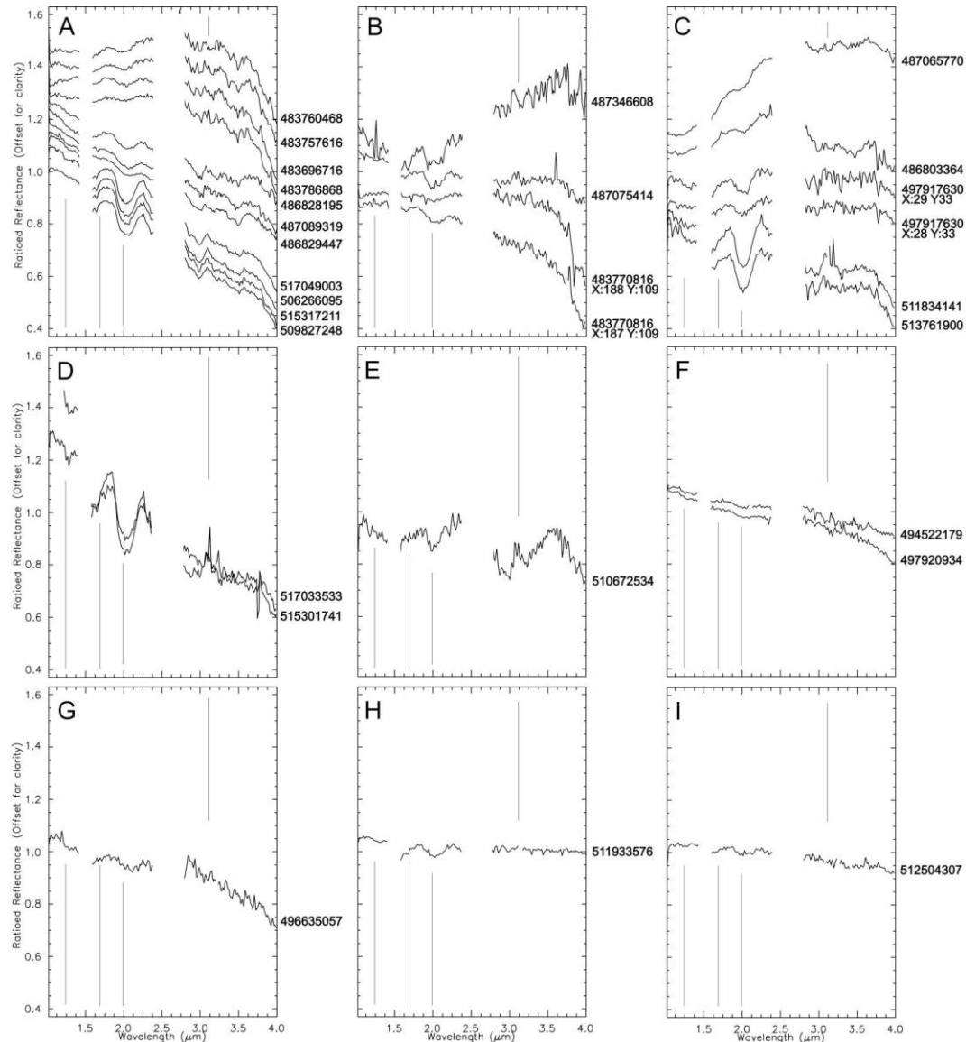
Fig. 5: Average ratioed and scaled reflectance VIR IR spectra of all H 2 O-rich areas identified on Ceres. Vertical gray lines indicate expected locations of H 2 O absorption bands at 1.28, 1.65 and 2.0 \mu\text{m} , as well as the position of the Fresnel peak of crystalline H 2 O ice 3.1 \mu\text{m} . A – (41.42°N, 0.76°E) Oxo Crater. B – (69.66°N, 114.81°E). C – (61.32°N, 221.06°E). D – (-34.83°N, 168.99°E) Juling Crater. E – (61.57°N, 51.82°E) Flow feature (Schmidt et al., 2017). F – (29.60°N, 155.07°E). G – (-47.92°N, 265.46°E) Baltnay Catena. H – (42.20°N, 199.51°E). I – (44.61°N, 32.50°E).
