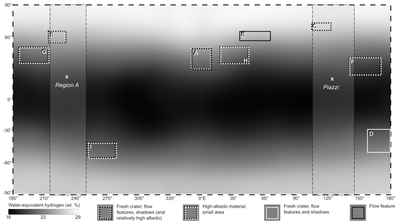
Fig. 16: Global distribution of water-equivalent hydrogen in the crust of Ceres from GROUND measurements (Prettyman et al., 2016) annotated with location of exposed H 2 O-rich areas detected by VIR. The rectangles indicate the boundaries of FC context images, similar to Fig. 2, and the line style refer to the type of surface feature that is observed. The grey vertical bands and locations marked by an X labeled Region A and Piazzzi refer to the two areas identified as possible sources of H 2 O vapor outgassing by Küppers et al. (2014). Projection: Simple Cylindrical; central meridian: 0.
