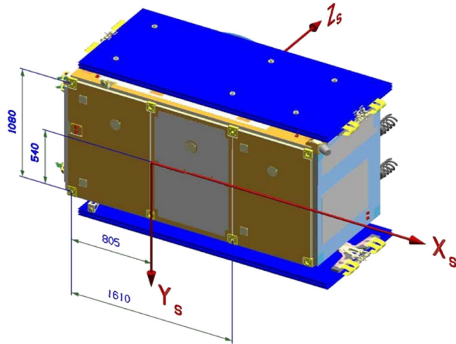
FIG. 1. Galileo FOC spacecraft: the mechanical reference frame. The MRF s aligned with the main body axes and originates in the separation plane of dispenser and satellite in the exact middle of the four I/F point center lines. The +Z_s -axis is normal to the separation plane and points toward the L-band navigation antenna. The +X_s -axis is normal to the clock panel and points toward the clock panel. The +Y_s -axis completes the right-handed orthogonal system. Courtesy of ESA from Galileo metadata.
