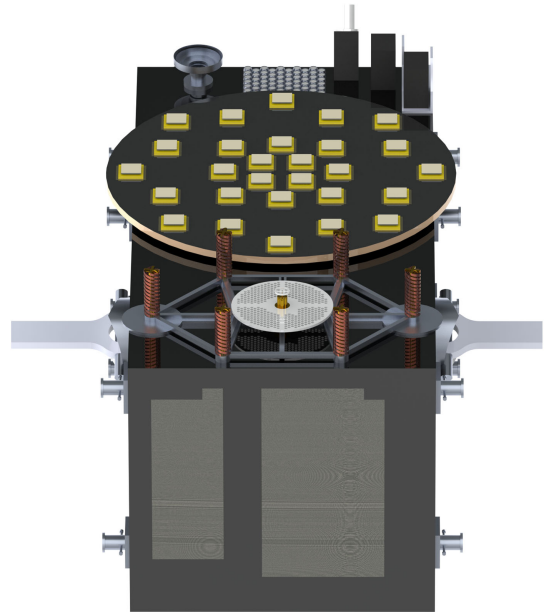
F4:1 FIG. 4. 3D-CAD model of a Galileo FOC spacecraft. The +Z F4:2 and +X surfaces are shown.
