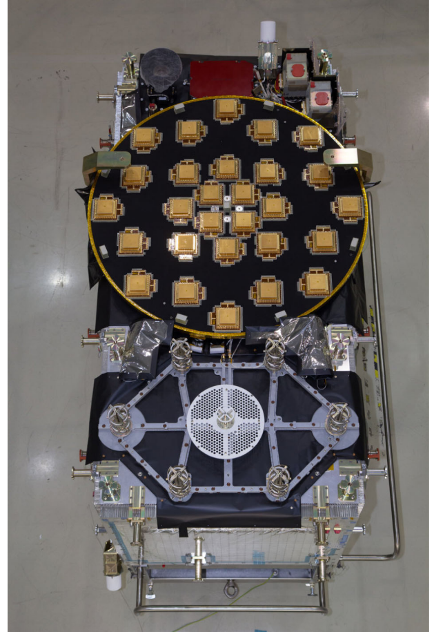
FIG. 2. Galileo FOC spacecraft: photo of the +Z panel. Courtesy of ESA.
