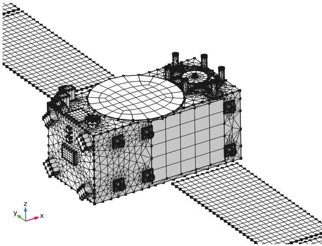
F6:1 FIG. 6. A very preliminary partial mesh of the 3D-CAD model F6:2 of a Galileo FOC spacecraft. The +Z, -X and -Y surfaces are F6:3 shown with part of the solar panels.
