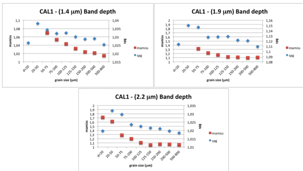
Figure 12. Sample CAL1. Band depth of absorptions at 1.4 \mu\text{m} (A), 1.9 \mu\text{m} (B), 2.2 \mu\text{m} (C).
