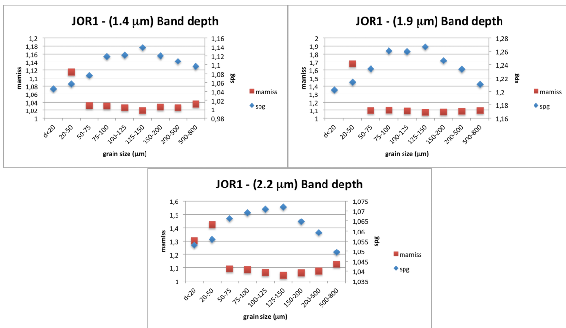
Figure 15. Sample JOR1. Band depth of absorptions at 1.4 \mu\text{m} (A), 1.9 \mu\text{m} (B), 2.2 \mu\text{m} (C).
