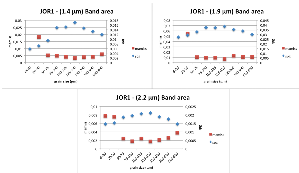
Figure 16. Sample JOR1. Band area of absorptions at 1.4 \mu\text{m} (A), 1.9 \mu\text{m} (B), 2.2 \mu\text{m} (C).
