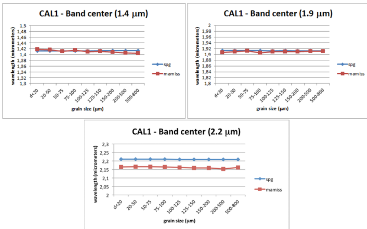
Figure 11. Sample CAL1. Band center of absorptions at 1.4 \mu\text{m} (A), 1.9 \mu\text{m} (B), 2.2 \mu\text{m} (C).
