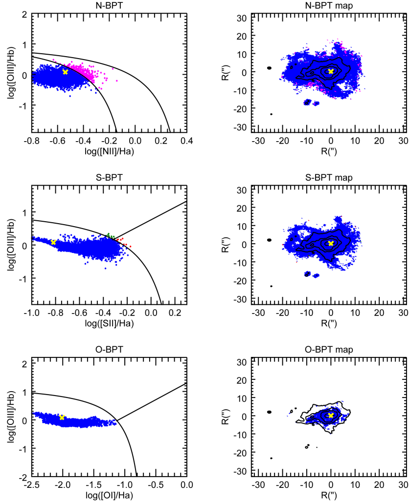
Fig. 5. Resolved BPT diagrams for He 2-10. The N-BPT diagrams for each spaxel with S/N > 3 in each line are shown on the left ; [\text{NII}]\lambda 6584/\text{H}\alpha vs. [\text{OIII}]\lambda 5007/\text{H}\beta are indicated in the upper panels , S-BPT diagrams [\text{SII}]\lambda 6716, 30/\text{H}\alpha vs. [\text{OIII}]\lambda 5007/\text{H}\beta in the central panels , and O-BPT diagrams [\text{OI}]\lambda 6300/\text{H}\alpha vs. [\text{OIII}]\lambda 5007/\text{H}\beta in the lower panels . The location of line ratios at the location of the nuclear radio source classified as accreting BH by Reines et al. (2011) are shown with a yellow cross. A map indicating each spaxel with the color corresponding to the dominant excitation at its location is shown on the right , again for spaxels with S/N > 3 . The star forming regions are indicated in blue, the Seyfert-type ionization is shown in green, LINER/shock dominated regions are shown in red, and intermediate regions are shown in magenta in the N-BPT. The contours of \text{H}\alpha line emission are overplotted in black and the location of the radio source is indicated with a yellow cross. All the line emission is dominated by star formation like ionization in He 2-10, including at the location of the compact radio source.
