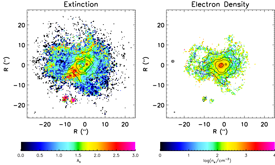
Fig. 4. Extinction map as derived from the H\alpha/H\beta line ratio ( left panel ) and electron density from [\text{SII}]\lambda 6716/[\text{SII}]\lambda 6730 ( right panel ) with H\alpha contours overplotted. Both maps show the spaxels with S/N > 3 in all the emission lines involved.
