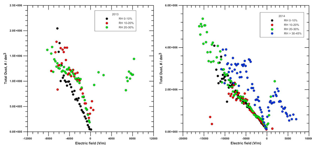
Figure 3. Relation between suspended dust concentration and E-field intensity for the (left) 2013 and (right) 2014 campaigns.
