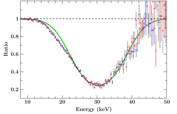
Figure 3. Residuals of observation 1 in terms of data-to-model ratio. The ratio was calculated by setting the strength of both absorption features to zero. FPMA data are shown in red, FPMB in blue. The best-fit model is shown in gray. The green line shows the ratio when only setting the second absorption feature to zero, i.e., when assuming a symmetric line profile. The data were strongly rebinned for the plot.
