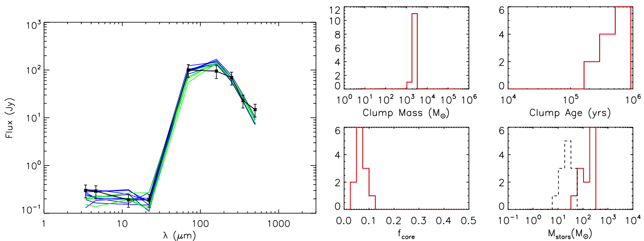
Figure 16. Same as Fig. 15 for IRAS05137+3919.
