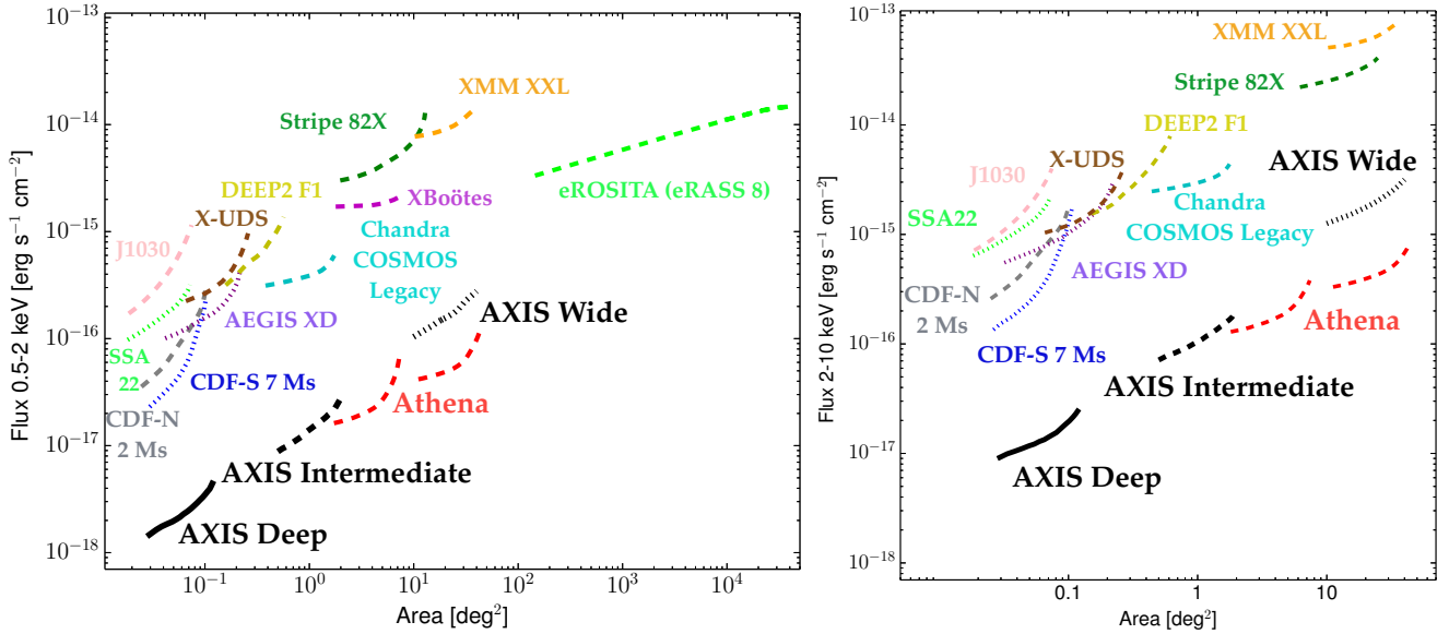
Fig. 10. 0.5–2 keV (left) and 2–10 keV (right) area-flux curves for the AXIS deep, 5 Ms (solid black line), intermediate, 300 ks (dashed black line) and wide, 15 ks (dotted black line) reference surveys. For comparison, we show the area-flux curves of several existing X-ray surveys: CDF-S 7 Ms (Luo et al. 2017, dotted blue line); CDF-N 2 Ms (Xue et al. 2016, dashed gray line); AEGIS XD (Nandra et al. 2015, dotted purple line); SSA22 (Lehmer et al. 2009, dotted light green line); XDEEP-2 F1 (Goulding et al. 2012, dashed yellow line); J1030 (dashed pink line; Nanni et al. 2020); X-UDS (Kocevski et al. 2018, dashed brown line); Chandra COSMOS Legacy (Civano et al. 2016, dashed cyan line); X-Bootes (Murray et al. 2005, dashed magenta line); Stripe 82X (LaMassa et al. 2013b,a, 2016, dashed green line); and XMM-XXL (Pierre et al. 2016, dashed orange line). We also show the predictions made for the ATHENA deep- and wide-area survey (dashed red lines; see the text for more details), and those for four years of eROSITA observations (i.e., eRASS:8; Merloni et al. 2012; Comparat et al. 2019, dashed light green line). The plotted lines have been derived from the 0.5–2 keV survey sensitivity curves in an area range that starts at 20% and stops at 80% of the area covered by the survey.
