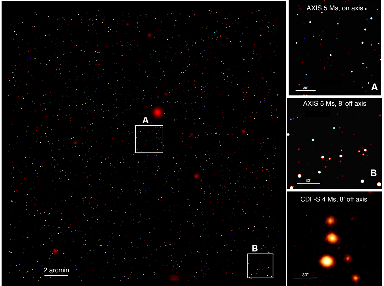
Fig. 8. Left: smoothed three-color image (red: 0.5–2 keV; green: 2–4.5 keV; blue: 7 keV) of a simulated 5-Ms deep field ( 24' \times 24' ) with AXIS. The extended red structures are galaxy clusters. The white boxes highlight two regions, one on-axis and the one at the boundary of the field of view: we show a zoom-in of these regions in the top and central right panels . The AXIS PSF is expected to have remarkably small degradation as a function of the off-axis angle. In the bottom right panel, we show as a reference a \sim 2' \times 2' , 8' off-axis 0.5–7 keV image of the 4 Ms CDF-S.
