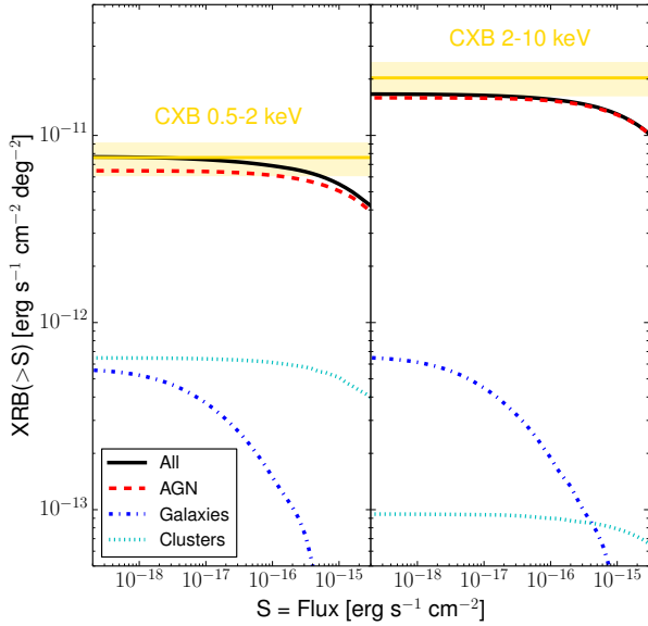
Fig. 5. Cumulative 0.5–2 keV (left) and 2–10 keV (right) fluxes per unit of square degree of the AGNs (dashed red line), nonactive galaxies (dash-dotted blue line) and galaxy clusters (dotted cyan line) simulated for the mocks used in this work. The overall distribution is plotted as a solid black line. The flux of the cosmic X-ray background measured by Cappelluti et al. (2017) is plotted in yellow, with 20% errors to account for the uncertainties in the CXB absolute flux level measured by different instruments.
