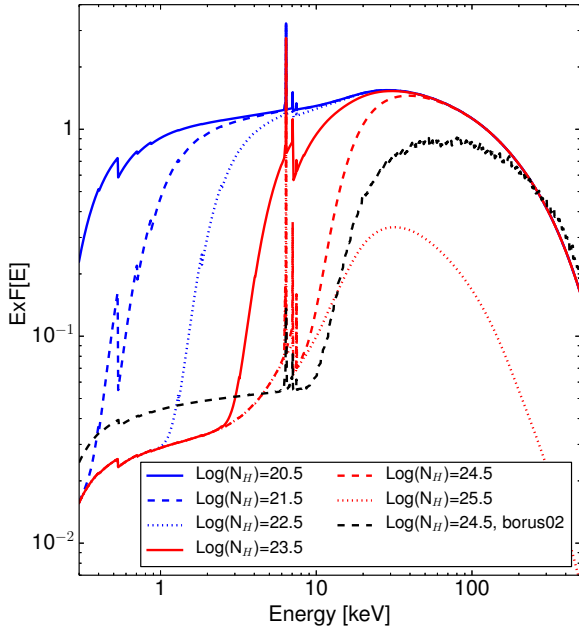
Fig. 3. AGN spectra used in our simulations, at z = 0 and for different \log(N_H) values. We also plot the spectrum of a CT-AGN with \log(N_H) = 24.5 as modeled using the borus02 model (Baloković et al. 2018, dashed black line), as a reference.
