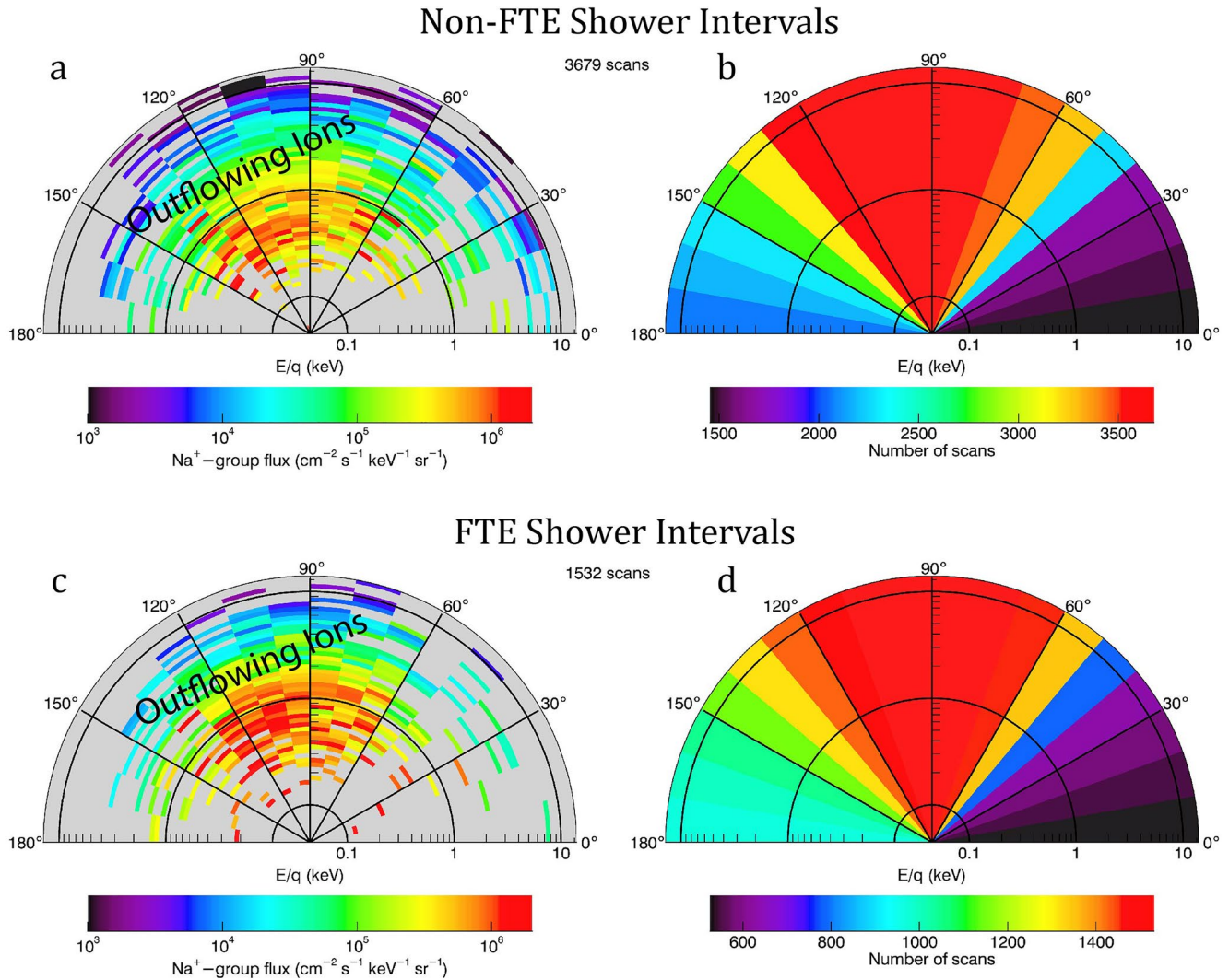
Figure 7. Fast Imaging Plasma Spectrometer (FIPS) measurements of the pitch angle-energy distribution of the Na + -group ions near the planet's surface beneath the northern cusp. The integration areas include magnetic local time (MLT) from 09:00 to 15:00, magnetic latitude (MLAT) from 55° to 70°, and altitude from 0 to 244 km ( 0.1 R_M ). The pitch angle bin size is 10°. Upper panels (a, b) are for the non-FTE shower intervals and lower panels (c, d) are for flux transfer event (FTE) shower intervals. Panels on the left (a, c) show the distributions of the differential particle flux ( \text{cm}^{-2} \text{s}^{-1} \text{keV}^{-1} \text{sr}^{-1} ). Panels on the right (b, d) show the distributions of the number of scans made by FIPS in each pitch angle bin.
