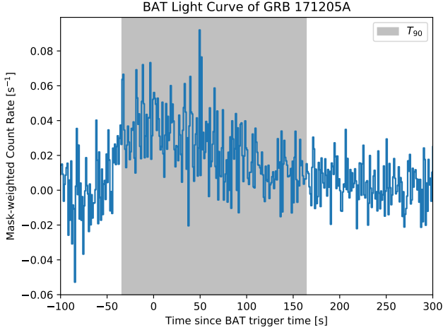
Fig. 1. Swift /BAT mask-weighted light curve in 15–350 keV and 1 s time bins. The gray region encloses the T_{90} interval.
