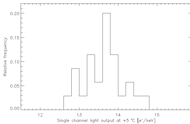
Figure 15 Single channel light output measured at T = +5\text{ }^{\circ}\text{C} at 662 keV
