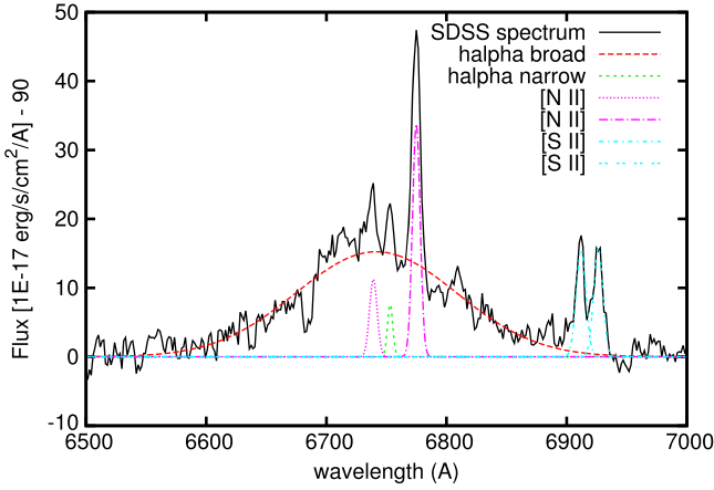
Figure 5. Fit to the H\alpha broad emission line and blended narrow lines in the SDSS DR9 optical spectrum of NGC 6418. The fitted Gaussian profiles represent: broad H\alpha (red), [N II]\lambda\lambda 6548, 83 (magenta), and [S II]\lambda\lambda 6717, 31 (cyan) and narrow H\alpha (green).
