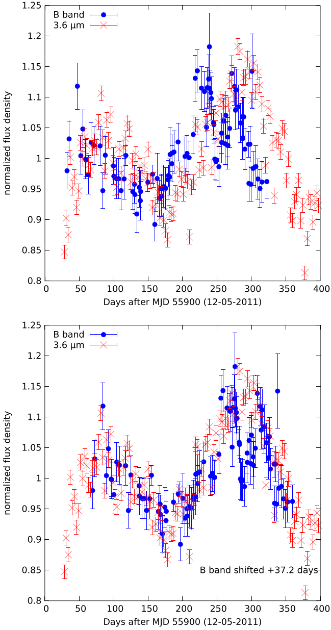
Figure 1. Spitzer 3.6 \mu\text{m} and the combined B band optical light curves. The error bars of the 3.6 \mu\text{m} and the combined B band optical light curves are the uncertainties reported by MOPEX and the image differencing solution, respectively. The bottom panel shows the combined optical light curve shifted by +37.2 days.
