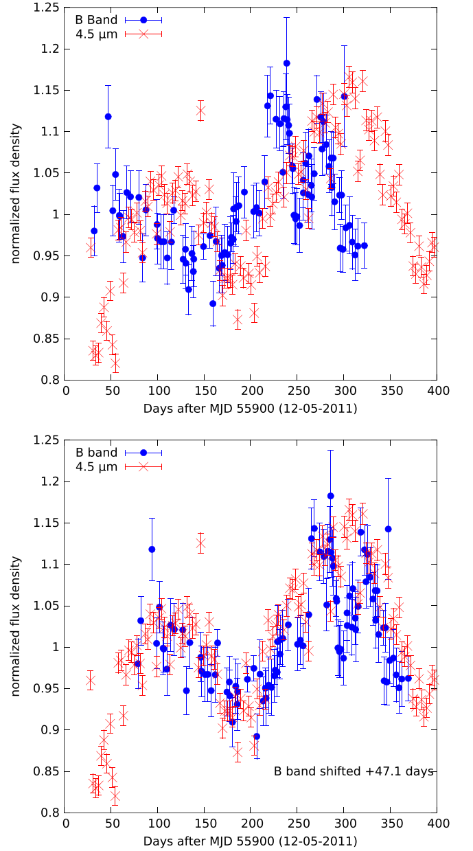
Figure 2. Spitzer 4.5 \mu\text{m} and the combined B band optical light curves. The error bars of the 4.5 \mu\text{m} and the combined B band optical light curves are the uncertainties reported by MOPEX and the image differencing solution, respectively. The bottom panel shows the combined optical light curve shifted by +47.1 days.
