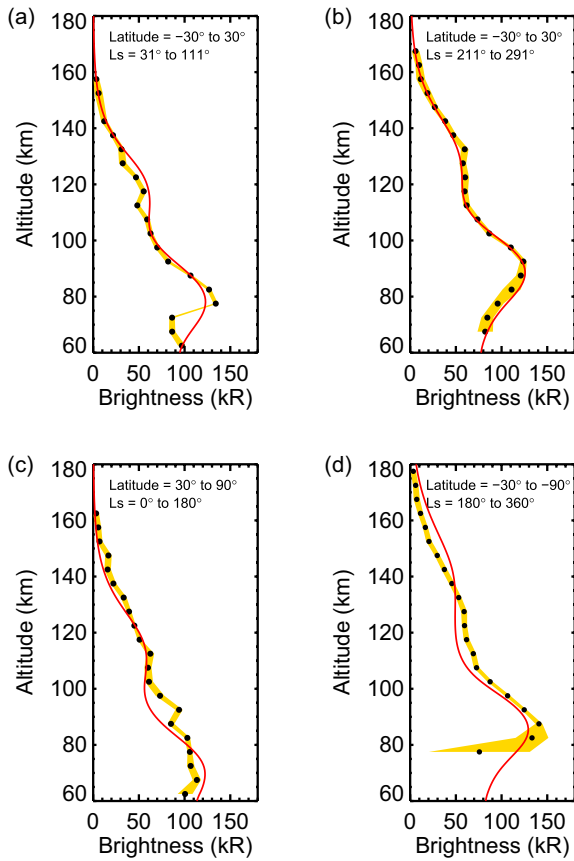
Figure 7. Averaged Ultraviolet and Visible Spectrometer limb profiles of the oxygen green line emission (black dots) acquired between 24 April 2019 (MY 35, L_s = 15^\circ ) and 31 December 2021 (MY 36, L_s = 150^\circ ). (a) Near aphelion in the equatorial region (based on a total of 825 spectra), (b) near perihelion in the equatorial region (based on a total of 337 spectra), (c) in northern spring and summer (based on a total of 954 spectra), (d) in southern spring and summer (based on a total of 465 spectra). Because observations end at L_s = 150^\circ for MY 36, only MY 35 data are shown in panel (b) and (d). The mean SZA of the four limb profiles vary between 55^\circ and 60^\circ . Uncertainties on the brightness estimates are colored in yellow. Simulations of the Photochemical Airglow Mars model for the same conditions are overplotted in red (see Section 7.2.3).
