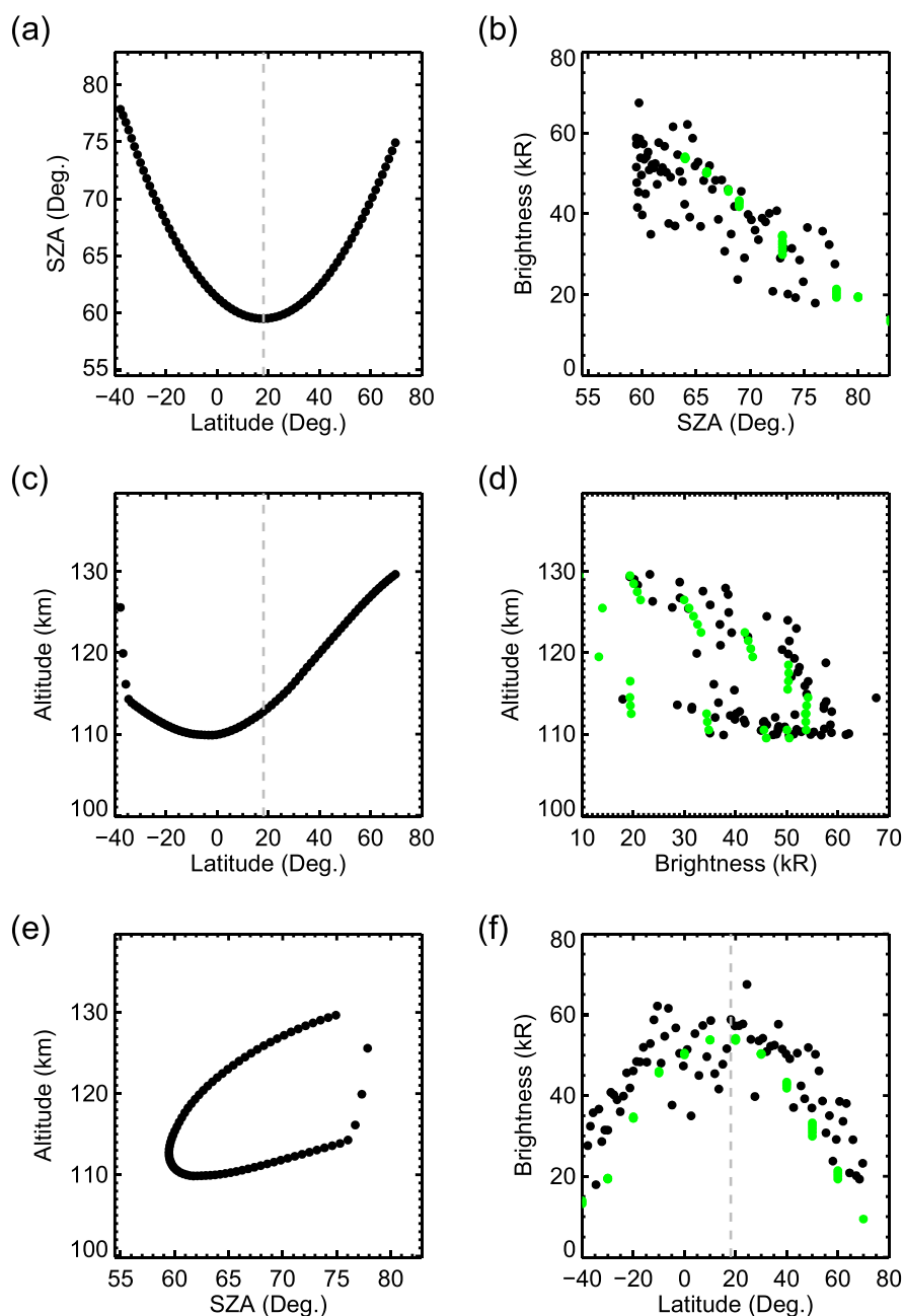
Figure 10. Nadir and Occultation for MArS Discovery/Ultraviolet and Visible Spectrometer limb tracking observation acquired on the 15 February 2021 ( L_s = 4^\circ ) based on 78 spectra (black dots). The left panels represent the geometry of the observation, scanning the Mars atmosphere at almost fixed altitude \sim 120 km (upper peak of the green line) from 40^\circ\text{S} to 70^\circ\text{N} . The vertical dashed lines in panels (a) and (c) represent the latitude where the SZA is minimum. The right panels show the brightness evolution of the green line as a function of SZA, altitude and latitude. Model simulations are shown with green dots.
