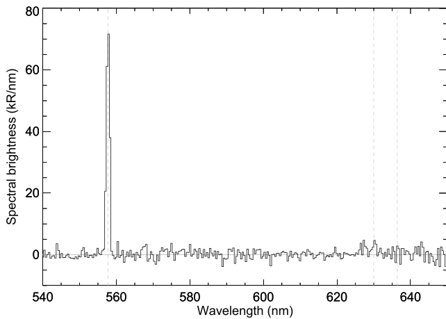
Figure 2. Average visible spectrum from Nadir and Occultation for Mars Discovery/Ultraviolet and Visible Spectrometer spectra obtained from 2531 spectra acquired between 75 and 140 km, for \text{SZA} < 70^\circ and all L_s . Vertical dashed lines represent the predominant oxygen green line at 557.7 nm and the much fainter red line doublet at 630–636.4 nm.
