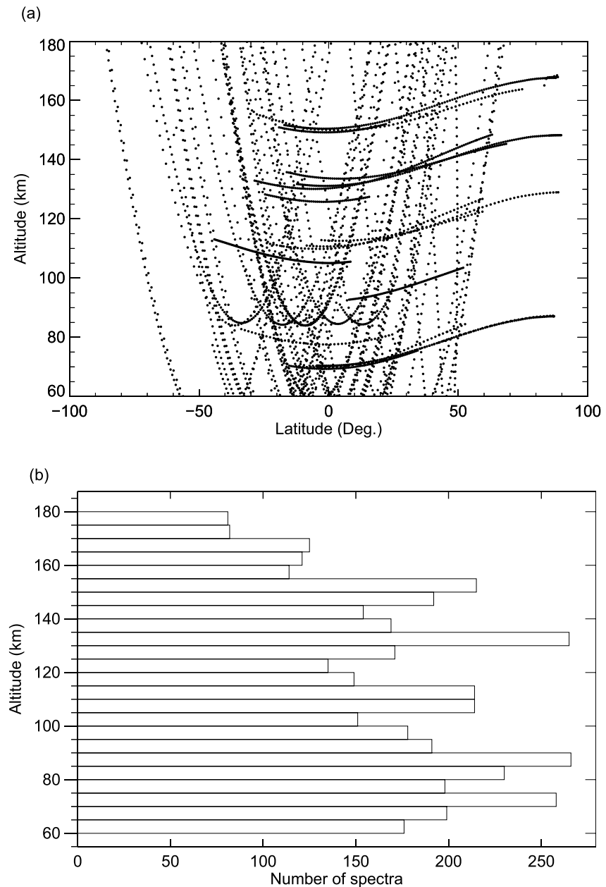
Figure 1. Limb data collected with Nadir and Occultation for MArS Discovery/Ultraviolet and Visible Spectrometer from 24 April 2019 (MY 35, L_s = 15^\circ ) to 31 December 2021 (MY 36, L_s = 150^\circ ) for solar zenith angles less than 70^\circ . (a) Inertial limb observations are characterized by a parabola shape while limb tracking observations are represented by the nearly horizontal lines (nearly constant altitude of the tangent point during the observation). (b) Altitude distribution of the 4248 spectra grouped in 5 km bins.
