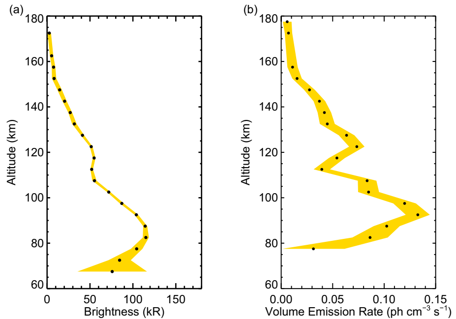
Figure 5. (a) global average limb profile of the [OI] 557.7 nm dayglow (black dots) retrieved from 4248 Nadir and Occultation for Mars Discovery/Ultraviolet and Visible Spectrometer spectra (see Figure 1). The emission peak is located at 82.5 km and reaches 115 kR. Uncertainties on the brightness estimates are colored in yellow. (b) Volume emission rate (VER) deduced from the profile shown in (a).
