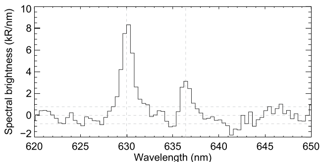
Figure 3. Average of 115 dayglow limb tracking spectra, essentially acquired during MY 36 ( L_s = 0-150^\circ ). Spectra are corrected from background noise, as explained in Section 3. The two components of the \text{O}(^1\text{D} \rightarrow ^3\text{P}) transition can be seen. The vertical dashed lines indicate the wavelength of the two doublet components. The horizontal dashed lines show the \pm 1\text{-}\sigma deviation of the background noise in the spectral window.
