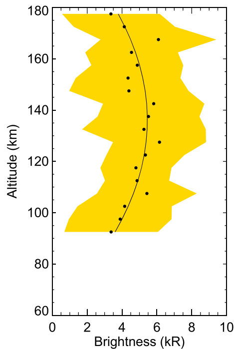
Figure 4. Average limb profile of the [OI] 630 nm dayglow (black dots) retrieved from 4248 spectra (see Figure 1) and best second order polynomial fit (black line). The emission maximum of the fit is located at 137.5 km and peaks at 5.3 kR. 1- \sigma uncertainties on the brightness estimates are colored in yellow.
