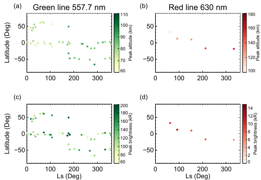
Figure 8. Variation of the peak altitude (top panels) and peak brightness (lower panels) of the oxygen green line (left panels) and red line (right panels) over seasons. Data points are generated using bins of 5° of solar longitude ( L_s ) and latitude for the green line. Bins of 15° of solar longitude are used for the red line.
