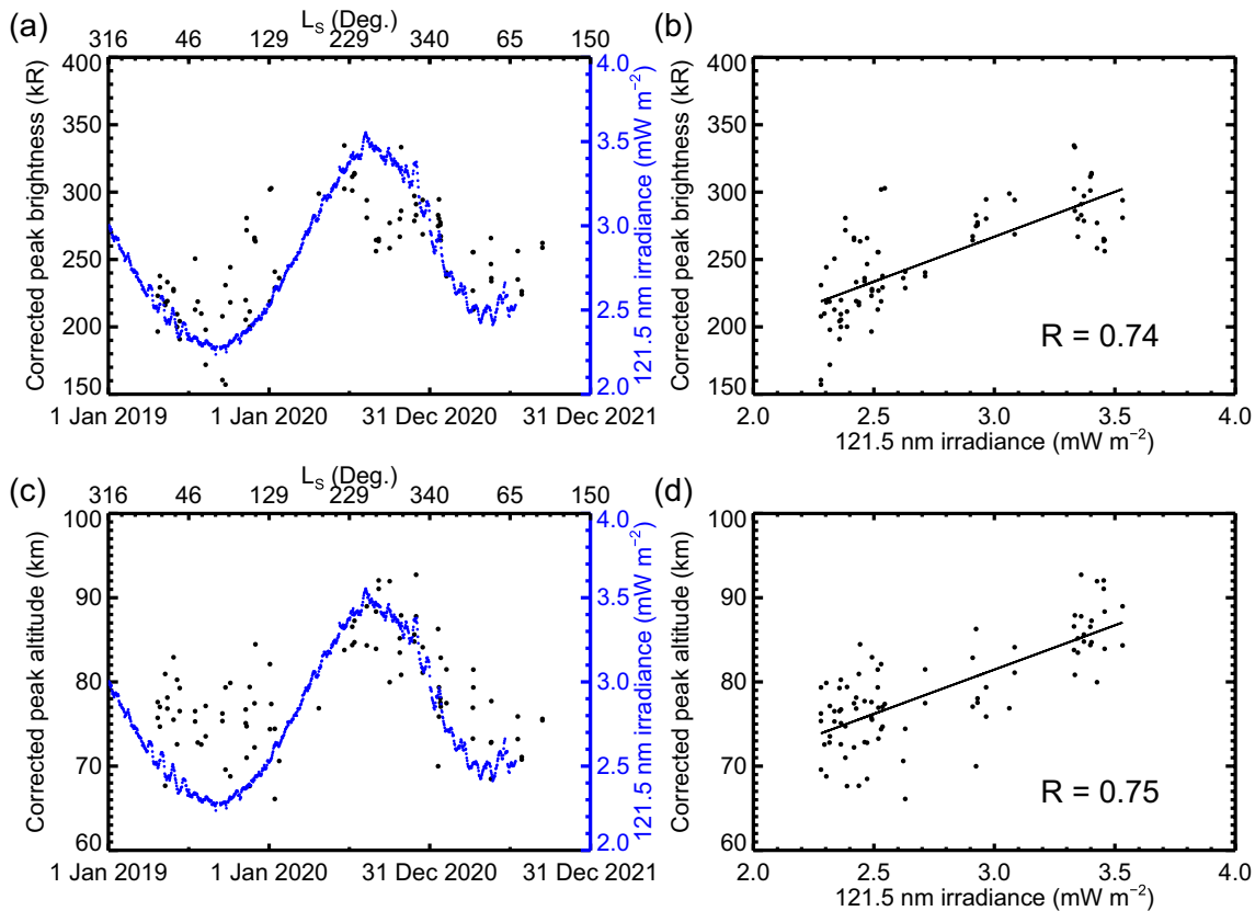
Figure 6. (a) Variation of the lower peak intensity of the oxygen green line along time (black dots). Intensities have been corrected from solar zenith angle (SZA) dependence. (b) A correlation with the Ly- \alpha irradiance (blue dots) can be observed. (c) Variation of the lower peak altitude of the oxygen green line along time (black dots). Altitudes have been corrected from SZA dependence. (d) A clear correlation with the Ly- \alpha irradiance (blue dots) can be observed.
