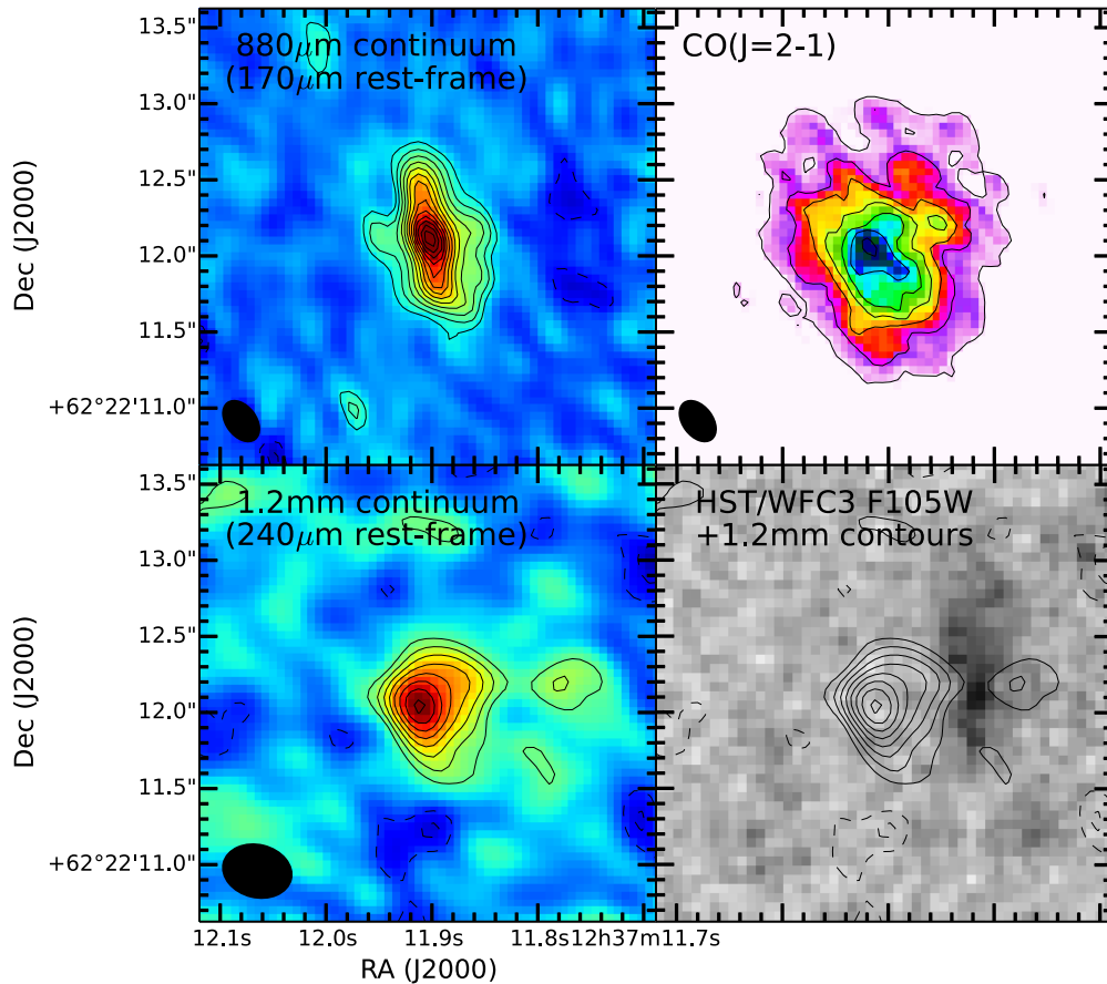
Figure 1. Multiwavelength imaging of the z = 4.05 SMG GN20. Top left: 880\text{ }\mu\text{m} PdBI image ( 0\text{'}.3 \times 0\text{'}.2 resolution). Contours start at \pm 2\sigma in steps of 1\sigma = 0.25\text{ mJy beam}^{-1} (corresponding to a rest-frame brightness temperature of T_B = 0.22\text{ K} ). The measured peak flux density of 3.6\text{ mJy} implies T_{B,\text{peak}} = 3.2\text{ K} . Top right: VLA CO(2–1) 0th moment map (H12) at the same resolution as the 880\text{ }\mu\text{m} data. Bottom left: 1.2\text{ mm} PdBI image ( 0\text{'}.46 \times 0\text{'}.35 resolution). Contours start at \pm 2\sigma in steps of 1\sigma = 0.25\text{ mJy beam}^{-1} . Bottom right: HST /WFC3 F105W image from the CANDELS survey (Grogin et al. 2011) and 1.2\text{ mm} contours.
