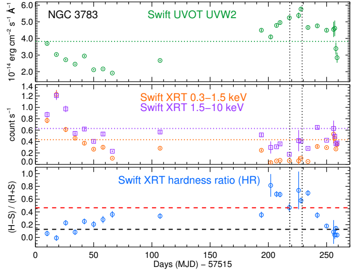
Fig. 1. Swift light curve of NGC 3783 from 17 May 2016 to 21 January 2017. The horizontal dotted lines in the two upper panels show the all-time average Swift flux levels. The dashed black line in the bottom panel indicates the average quiescent hardness ratio (HR) from unobscured data. The dashed line in red is the HR limit for triggering, above which significant obscuration was predicted according to our simulations. The first and second XMM-Newton observations are indicated by vertical dotted lines.
