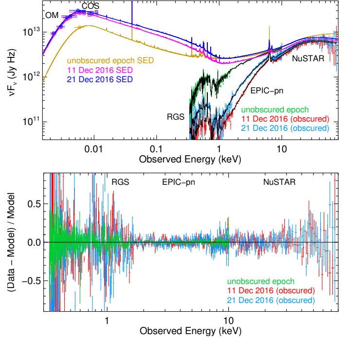
Fig. 6. Top panel: best-fit model to each dataset of NGC 3783, and its corresponding SED model. The displayed X-ray data include absorption by the Galaxy, the WA, and the obscurer. Bottom panel: residuals of the best-fit model.
