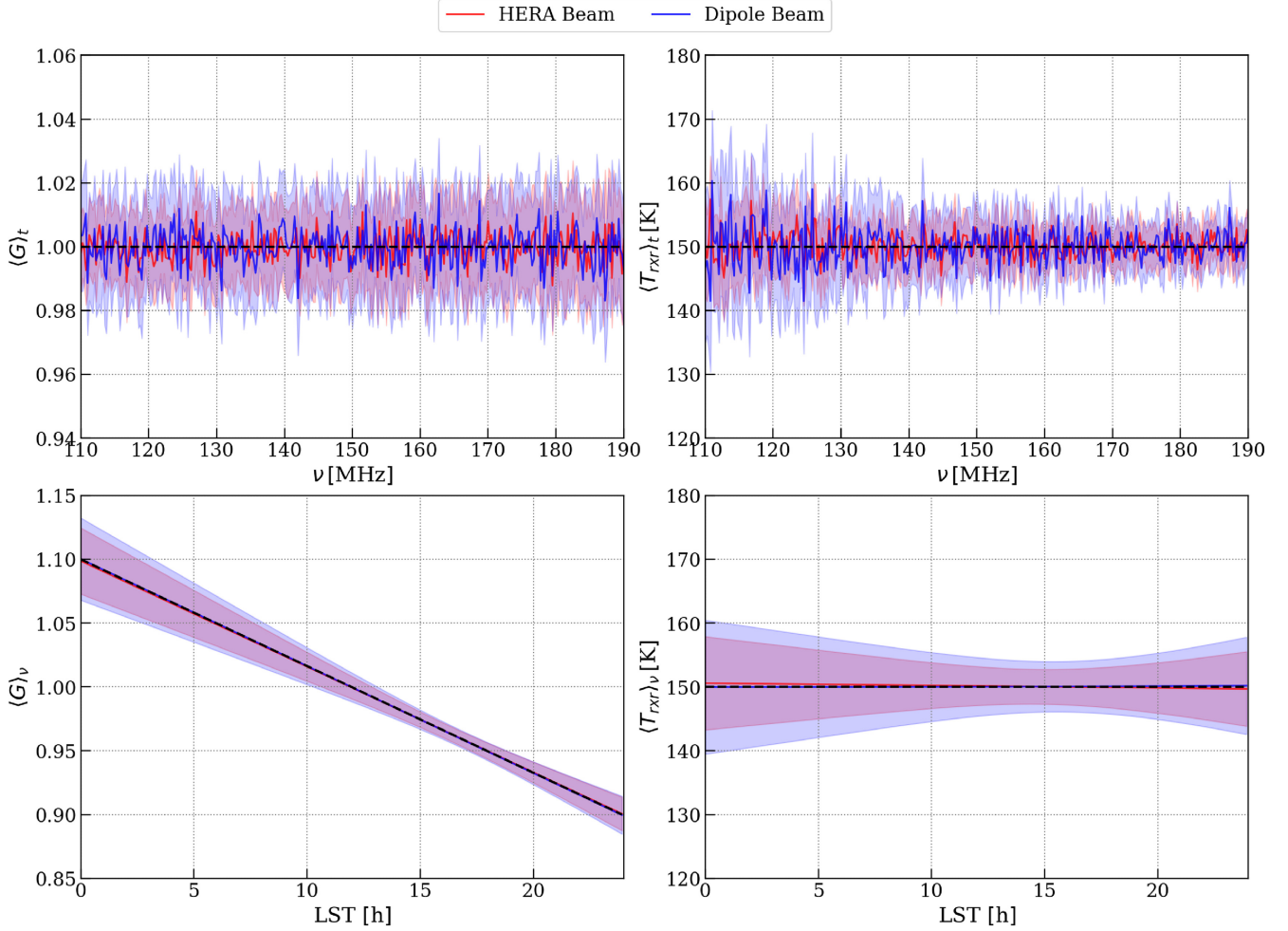
Figure 6. Calibration products for the modified calibration that uses first-order polynomials to fit for linear time-dependent gain G(t) (see Section 4.2). The top and bottom rows show calibration parameter \hat{G} (left-hand column) and \hat{T}_{\text{txr}} (right-hand column) averaged over time and frequency, respectively. Dashed lines show the input parameters averaged over corresponding axes. Shaded regions represent rms of error on the fit along the corresponding time and frequency axes used for averaging. Using a first-order polynomial in calibration mitigates the bias in calibration products due to temporal gain variations. However, corresponding uncertainty levels are increased relative to the reference case.
