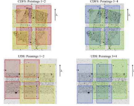
Fig. 2. Survey strategy. Four VIMOS pointings ( 4\times 7'\times 8'=224 \text{ arcmin}^2 each) for each field i.e., CDFS in the upper panels and UDS in the lower panels, designed to cover the whole HST area.
