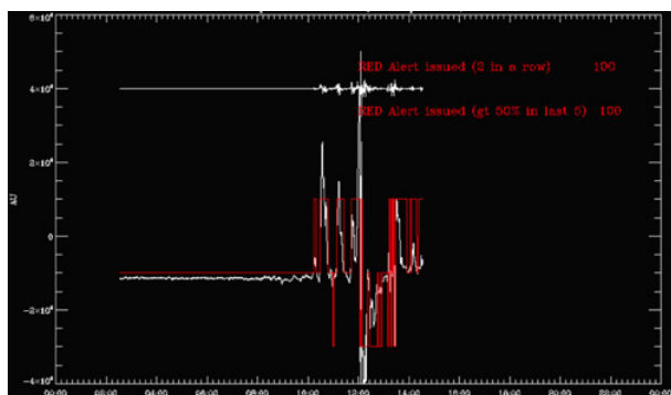
Figure 6. Alarm triggered using EFM signal on Jan. 5, 2014. Upper white line represents the derivative, lower white line the signal, red line indicate where alert was issued.
