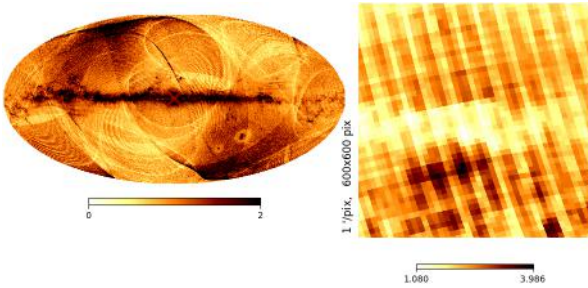
Fig. 30. Mean value of astrometric excess noise divided by parallax uncertainty. Left panel : whole sky. Right panel : 10^\circ size detail at the Galactic centre (0,0). Imprints of the scanning law are present throughout the whole sky.
