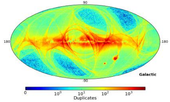
Fig. 1. Map of duplicated sources in Galactic coordinates.
