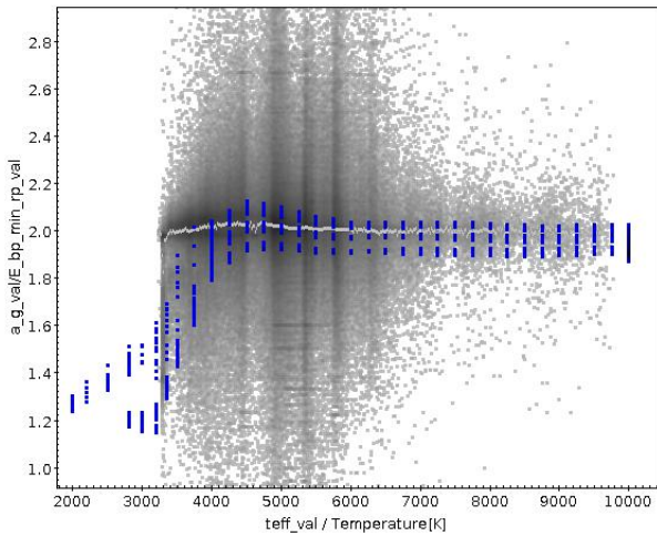
Fig. 52. Ratio A_G / E(G_{BP} - G_{RP}) as a function of T_{\text{eff}} as derived in DR2 (grey points). The grey line is a running median. Blue dots show the prediction using the stellar energy distribution of solar metallicity stars and the DR2 passbands (Evans et al. 2018).
