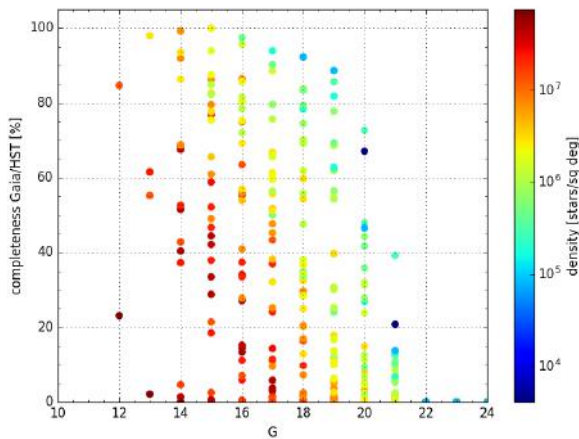
Fig. 7. Completeness levels with respect to HST data in different regions of 26 globular clusters with various local densities, showing the influence of crowding on the completeness.
