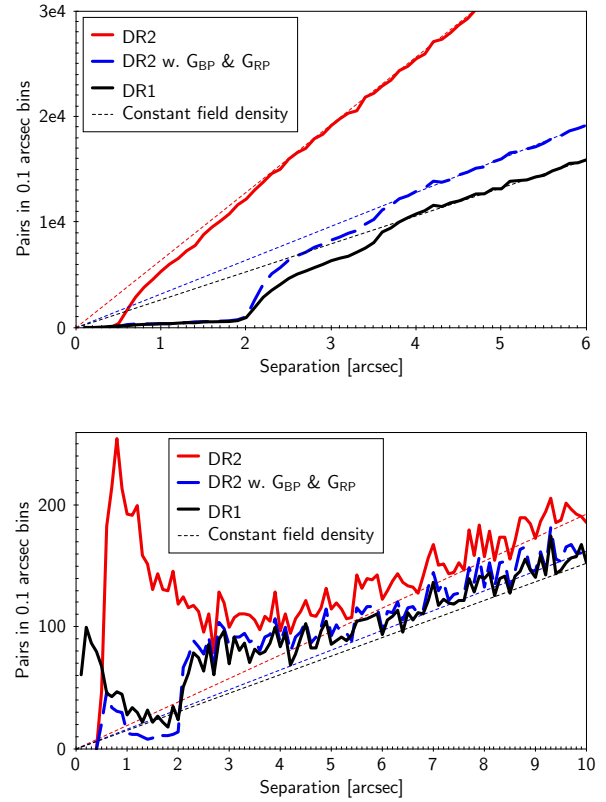
Fig. 9. Histogram of source pair separations in two test fields for Gaia DR2 sources, for Gaia DR2 sources with G_{BP} and G_{RP} photometry, and for Gaia DR1 sources. Top panel: dense field at (l, b) = (-30^\circ, -4^\circ) . Bottom panel: sparse field at (l, b) = (-100^\circ, -60^\circ) . The thin dotted lines show the relation for a random distribution.
