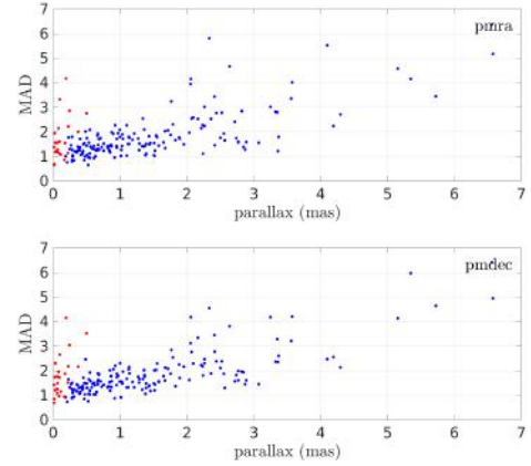
Fig. 26. MAD of the distribution of normalised differences on the proper motions ( \text{mas yr}^{-1} ) in right ascension ( top panel ) and declination ( bottom panel ) as a function of the parallax (in mas) for open clusters (blue dots) and globulars (red dots).
