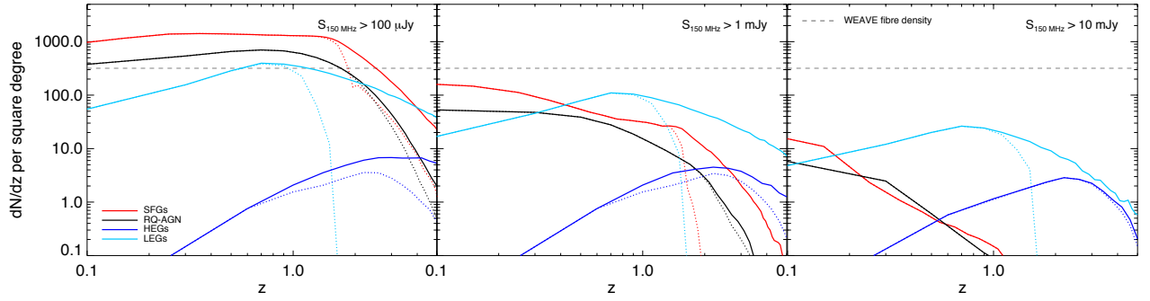
Fig. 4. The expected redshift distributions for each tier of WEAVE-LOFAR, including the Deep tier, at S_{150} > 100 \mu\text{Jy} ( Left ), the Mid tier ( S_{150} > 1 \text{ mJy} ; Centre ), and the Wide tier ( S_{150} > 10 \text{ mJy} ; Right ). Solid lines show the model redshift distribution while dotted lines of the same colour show the distribution of successful redshifts that we expect. The population has been divided to reveal the expected redshift distributions for each constituent of the source population according to the SKA Simulated Skies (Wilman et al. 2008), including star-forming galaxies (SFGs, in red), radio-quiet AGN (RQ-AGN, in black), high excitation radio galaxies (HEGs, in blue) and low-excitation radio galaxies (LEGs, light blue).
