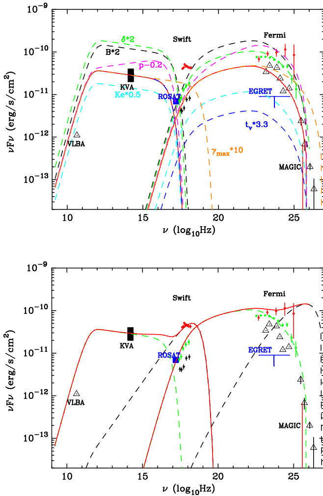
Figure 6. Spectral energy distribution of NGC 1275: the VLBA radio data of the C3 component (Suzuki et al. 2012), optical KVA data (Aleksić et al. 2014), ROSAT/HXI flux (Fabian et al. 2015) (filled rectangle), Swift in the normal (black, 00036524001 in 2007), high-flux (green, 00092034002 in 2015), and flare (red, 00031763002) states (this work), the LAT and MAGIC gamma-ray data in the normal (black) state (Abdo et al. 2009; Aleksić et al. 2014), high-flux (green), and flare (red) states (this work, the colors are the same as Figure 3). See the text for details. Solid and dashed lines are one-zone synchrotron self-Compton model curves calculated with the formula in Finke et al. (2008) for various parameter sets. Top: solid red line represents the baseline parameter set, and other dashed lines are curves which are based on the parameter set where only one parameter (as indicated on the plot) is changed from the baseline parameter set. Bottom: solid red line represents the double SSC model; one is for a steady component (green dashed) and the other is for a flare component (black dashed). See Table 3 for details.
