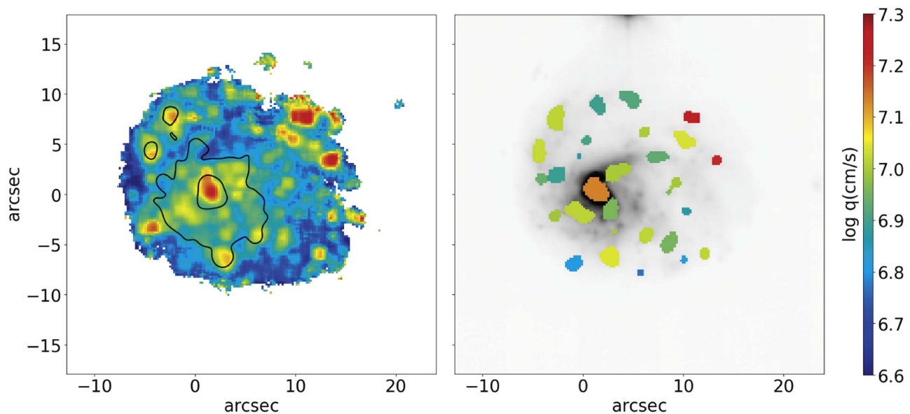
Figure 1. Ionization parameter ( q ) map. Left: contours represent the original body (see Figure 14 of Vulcani et al. 2018). Right: only regions corresponding to the 29 H \alpha knots identified in Figure 3 of Vulcani et al. (2018) are color coded according to the median q of each knots. In the background, the white-light image of the galaxy (Figure 2 of Vulcani et al. 2018) is shown, for reference.
