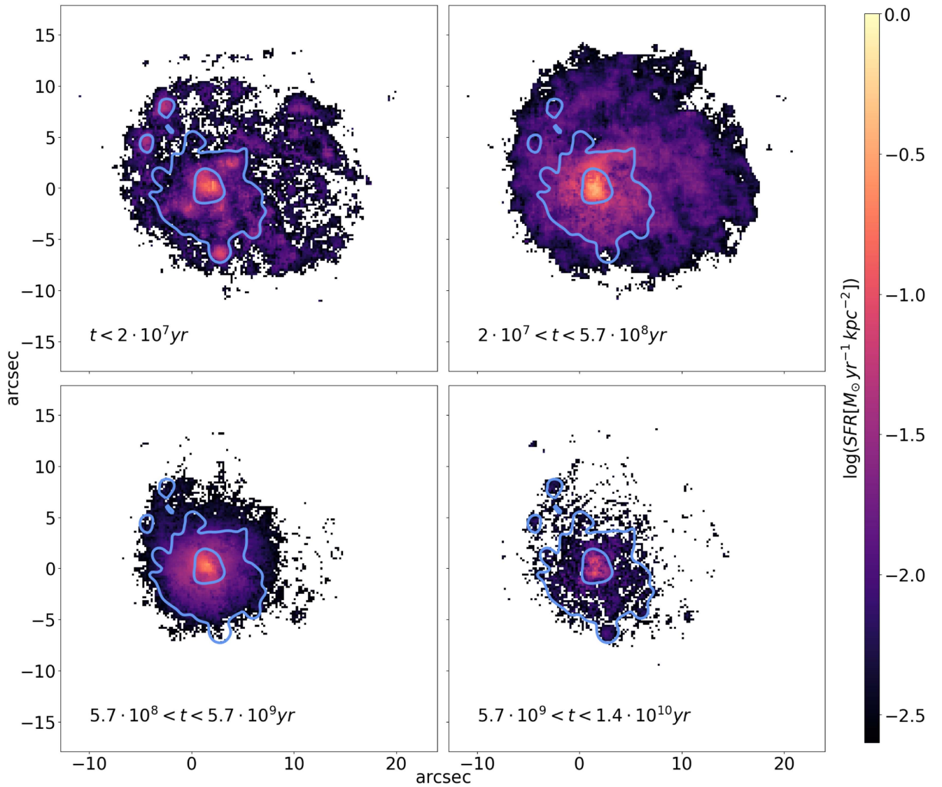
Figure 14. Stellar maps of different ages, illustrating the average star formation rate per \text{kpc}^2 during the last 2 \times 10^7 years (top left), between 2 \times 10^7 years and 5.7 \times 10^8 years (top right), 5.7 \times 10^8 years and 5.7 \times 10^9 years (bottom left), and > 5.7 \times 10^9 years ago (bottom right). Contours in all panels represent the original body, defined by the contours in the bottom right panel.
