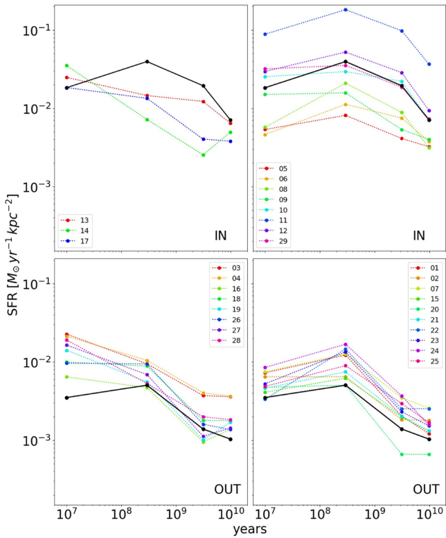
Figure 15. Star formation histories (average SFR in four age bins) per unit \text{kpc}^2 within (upper) and outside (bottom) the galaxy original body (see Figure 14), for each of the \text{H}\alpha knots (colored dashed lines). For the sake of clarity, the panels on the left show the \text{H}\alpha knots with rising SFH, and those on the right the \text{H}\alpha knots with declining SFH. The SFH for the entire galaxy within and outside the original body (black solid lines) is also reported for comparison.
