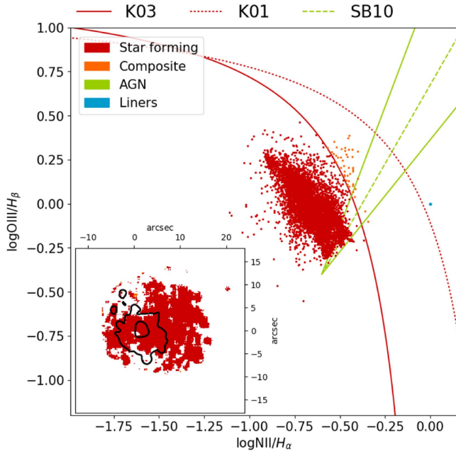
Figure 5. Diagnostic diagram for [O\ III]5007/H\beta vs. [N\ II]6583/H\alpha . Lines are from Kauffmann et al. (2003, K03), Kewley et al. (2001, K01), and Sharp & Bland-Hawthorn (2010, SB10) to separate star-forming, composite, AGN, and LINERS. In the inset, the BPT line-ratio map is shown. Only spaxels with an S/N > 3 in all of the emission lines involved are shown.
