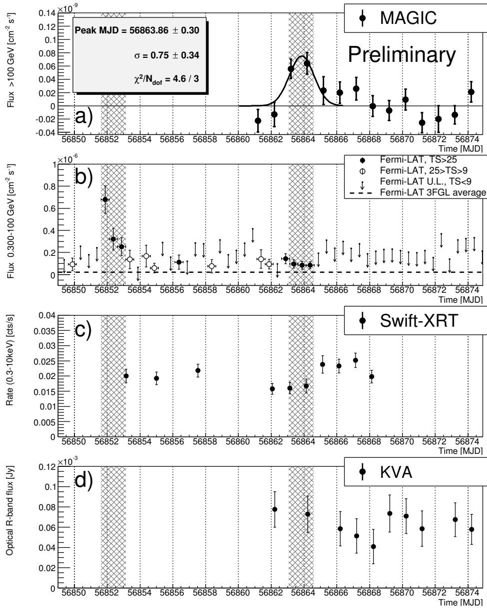
Figure 2. Multiwavelength light curve of QSO B0218+357 during the flaring state in July/August 2014. (a) MAGIC (points) above 100 GeV with a Gaussian fit to the peak position (thick solid line); (b) Fermi -LAT above 0.3 GeV with the average flux from the 3rd Fermi -LAT Catalog [22] shown as a dashed line. Notice that during the days where the trailing emission was expected Fermi -LAT was in pointing mode allowing significant detection of lower flux levels; (c) Swift -XRT count rate in the 0.3–10 keV range; (d) KVA in R band (not corrected for the contribution of host/lens galaxies and the Galactic extinction). The two shaded regions are separated by 11.46 days.
