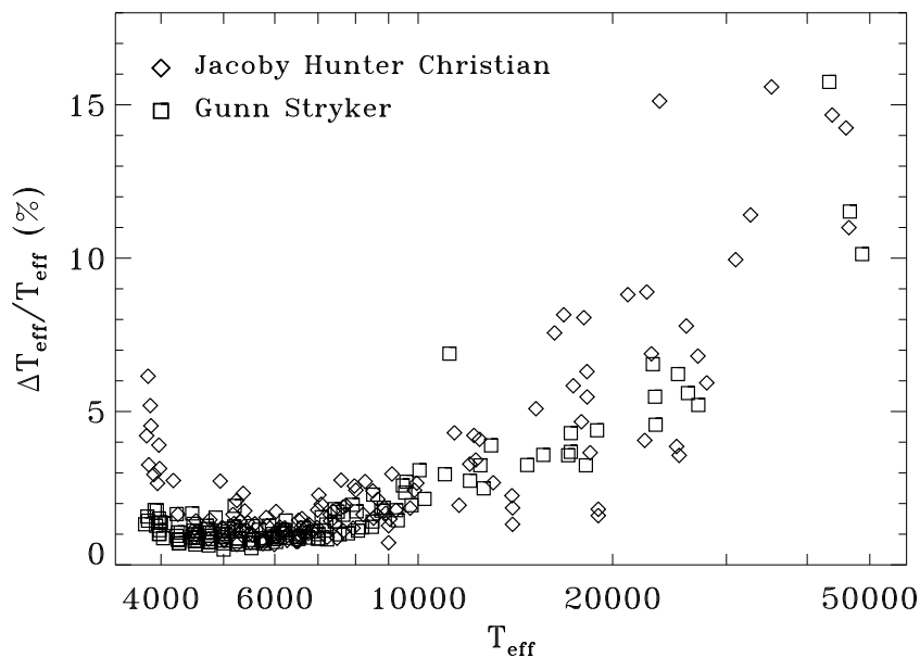
Fig. 3.— Relative error on the T_{\text{eff}} of the stars of the two atlases. The typical 2\text{-}\sigma absolute error is \pm 50\text{--}100\text{ K} for K–F stars, \pm 100\text{--}200\text{ K} for A stars and \pm 400\text{--}1000\text{ K} for B stars.
