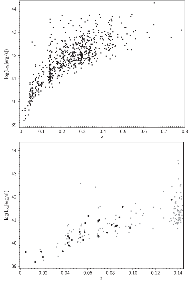
Figure 2. Plot of soft-band X-ray luminosity L_{Xs} against redshift z for the same objects as in Fig. 1. Lower panel: Expanded version showing only the galaxies at redshifts out to z = 0.145 , approximately the limit for our low-mass sample. The latter are shown as filled circles.
