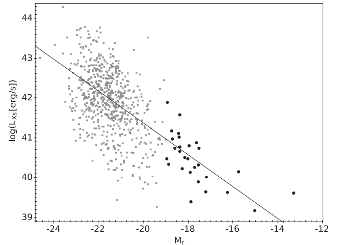
Figure 3. Plot of soft-band X-ray luminosity L_{Xs} against absolute r -band magnitude M_r for the same objects as in Fig. 2. Low-mass galaxies are again the filled circles. The line indicates the approximate locus of AGN with an Eddington ratio of 10^{-2} (see text).
