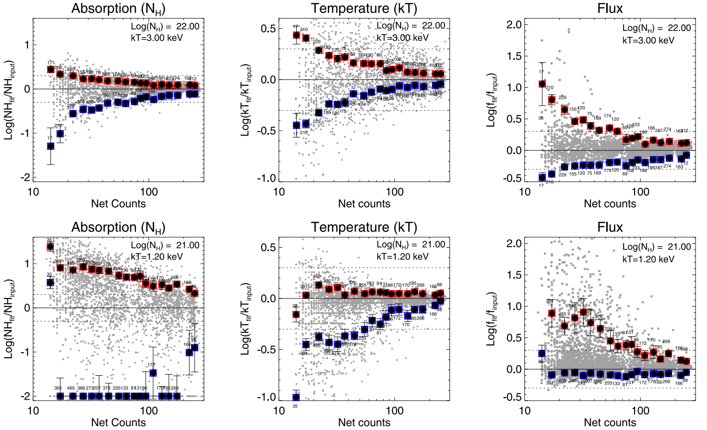
Figure 2. The relative errors in N_H , kT , and flux as a function of the input net counts imposed on the spectral simulations. The top panels correspond to a spectral model grid point \log(N_H) = 22.00 and kT = 3.0 keV, and the bottom panels correspond to a model with \log(N_H) = 21.00 and kT = 1.20 keV. The red and blue boxes refer to the Q uncertainty computed for the relative error distributions (gray circles) for each incremental range in photon counts in which we simulate the spectra. The numbers next to these points indicate the number of simulations included in each respective bin. We point out that relative errors for N_H in the bottom middle panel artificially bottom out at an N_H value a factor of 100 lower than the input value for cases of less than about 100 net source counts. This numerical conditioning is imposed in order to avoid unconstrained lower limit values of N_H for low column density cases (see also Section 3).
