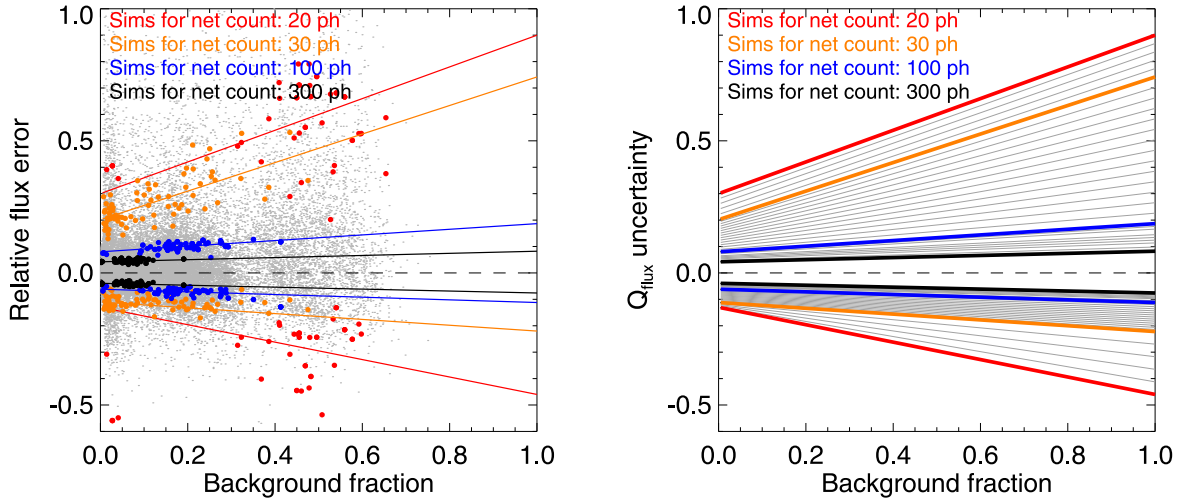
Figure 5. The left panel illustrates curves fitted to the relative flux error as a function of the background fraction for the thermal model 1 ( N_H = 1.0 \times 10^{22} , kT = 3.0 ) according to MC simulations containing 20 (red), 30 (orange), 100 (blue), and 300 (black) net photons in the spectra, respectively (see text). Large colored circles in the panel are the quantile uncertainties for flux. The relationship between the flux uncertainty and background fraction is clearly quite linear. The right panel illustrates the synthesis of the fits to the data of the left panel. The whole set of interpolated curves for the rest of the model parameters investigated and for each of 14 models was computed but not shown here. The same numerical treatment was performed for nonthermal models and for all spectral parameters.
