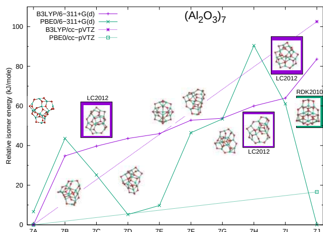
Fig. 9. Relative energies of the lowest-energy alumina heptamer isomers ( \text{Al}_2\text{O}_3 ) 7 . Structures reported by Li & Cheng (2012) are indicated in violet as LC2012 and the GM candidate reported by Rahane et al. (2011) in green as RDK2010.
