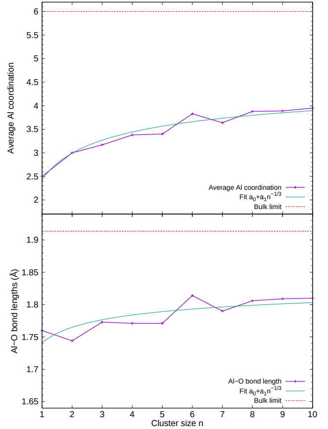
Fig. 29. Average Al coordination (top panel) and average AlO bond length in the GM clusters as a function of cluster size, n . The values for the bulk limit ( \alpha -alumina) are given in dashed red lines.
