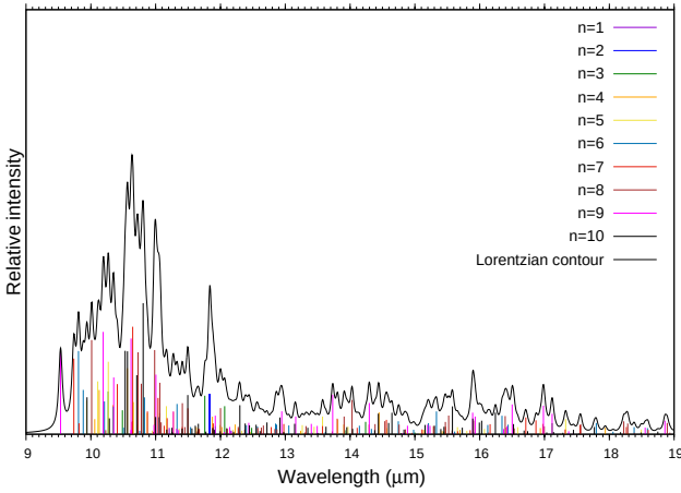
Fig. 30. Vibration modes of the (\text{Al}_2\text{O}_3)_n , n = 1-10 , GM clusters (colour-coded) as a function of the wavelength (in \mu\text{m} ). The black contour corresponds to non-weighted (in size and metastable isomers) Lorentzian distribution.
